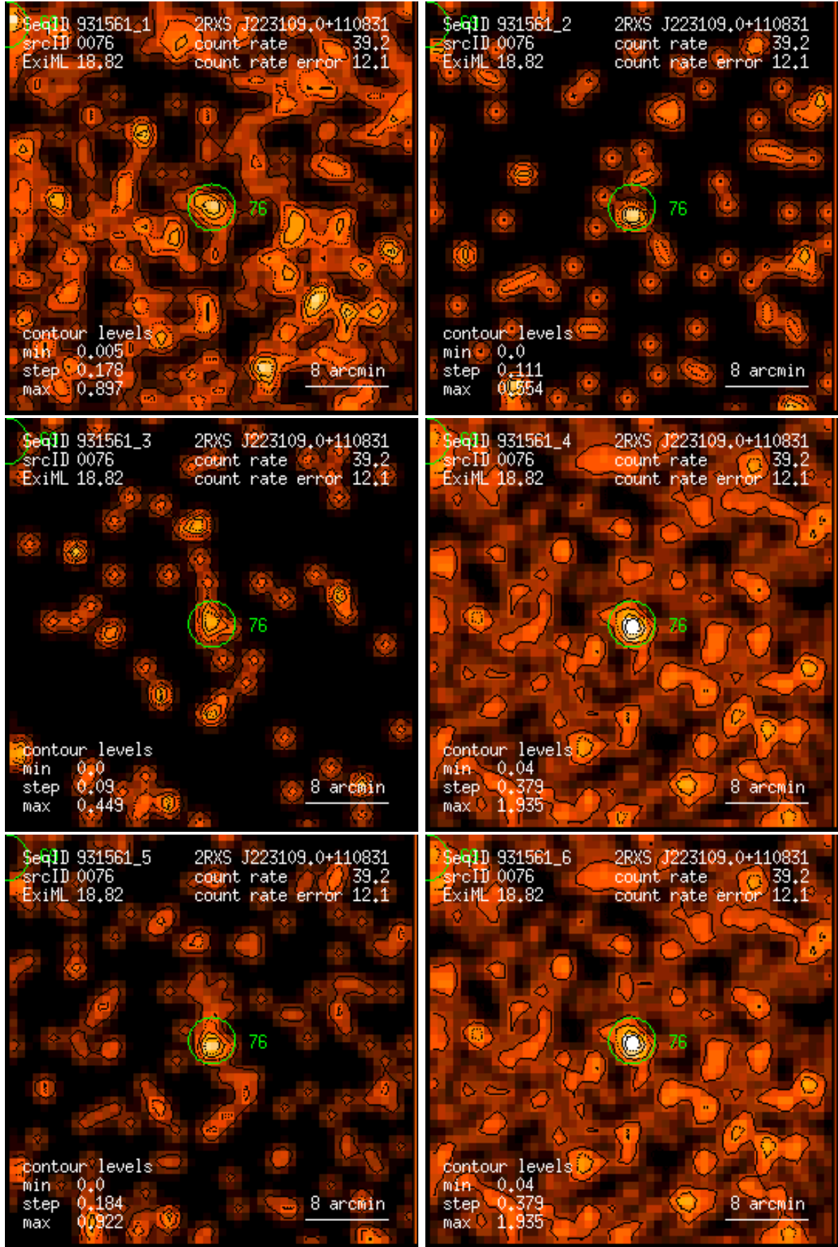
Figure 76: RASS 931561: detection 0076: band rate images, Gaussian filter: (1) PSPC channels 11 – 41, (2) 52 – 90, (3) 91 – 201, (4) 11 – 235, (5) 52 – 201, (6) 11 – 201. Broad band rates in counts/ks. Band rate contour levels in counts/ks/arcmin 2 .
