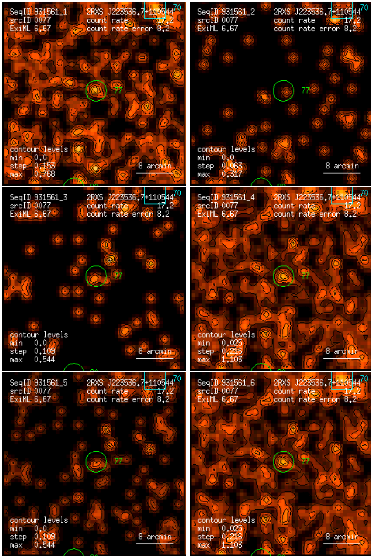
Figure 77: RASS 931561: detection 0077: band rate images, Gaussian filter: (1) PSPC channels 11 – 41, (2) 52 – 90, (3) 91 – 201, (4) 11 – 235, (5) 52 – 201, (6) 11 – 201. Broad band rates in counts/ks. Band rate contour levels in counts/ks/arcmin 2 .
