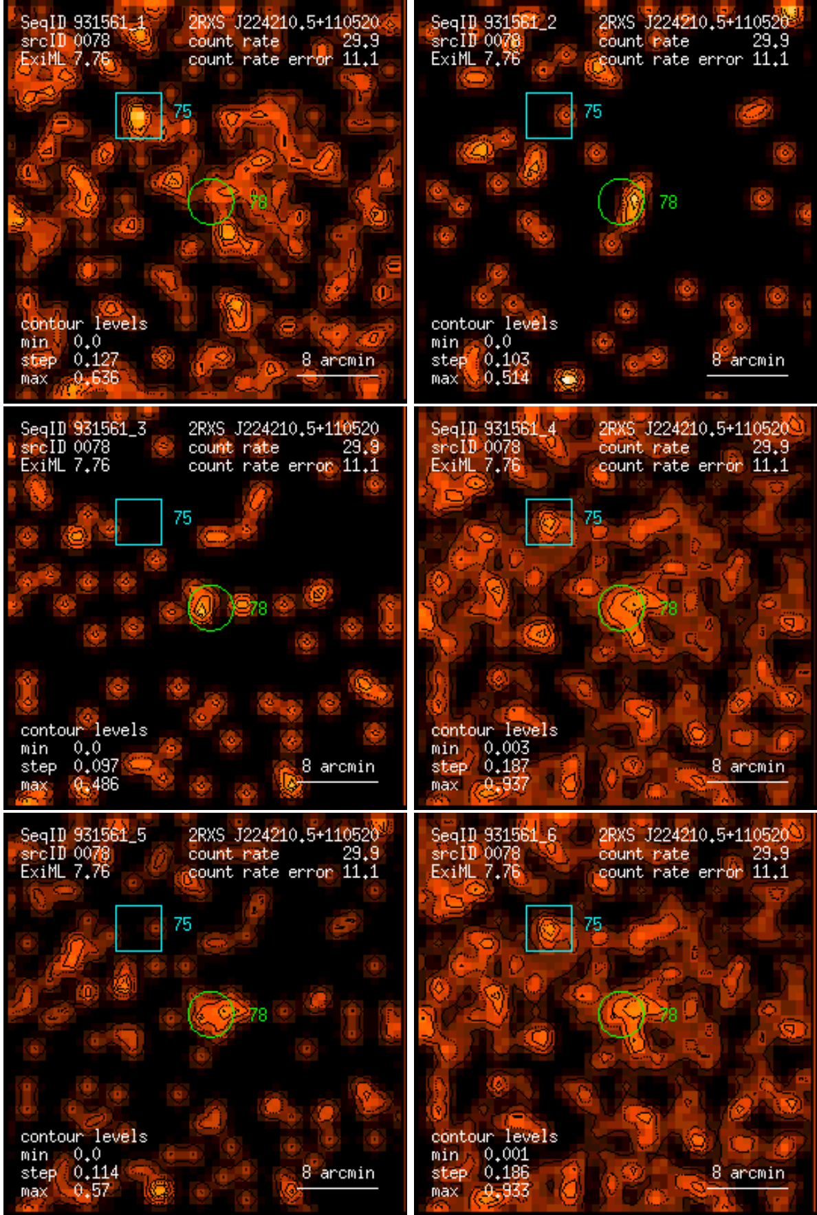
Figure 78: RASS 931561: detection 0078: band rate images, Gaussian filter: (1) PSPC channels 11 – 41, (2) 52 – 90, (3) 91 – 201, (4) 11 – 235, (5) 52 – 201, (6) 11 – 201. Broad band rates in counts/ks. Band rate contour levels in counts/ks/arcmin 2 .
