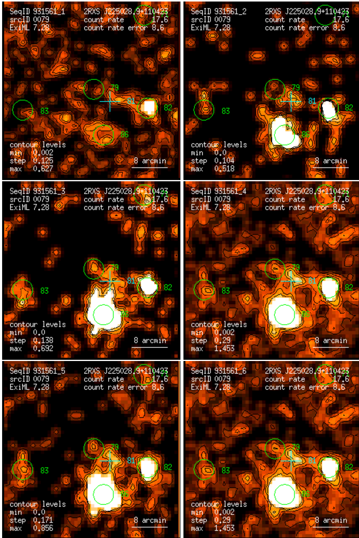
Figure 79: RASS 931561: detection 0079: band rate images, Gaussian filter: (1) PSPC channels 11 – 41, (2) 52 – 90, (3) 91 – 201, (4) 11 – 235, (5) 52 – 201, (6) 11 – 201. Broad band rates in counts/ks. Band rate contour levels in counts/ks/arcmin 2 .
