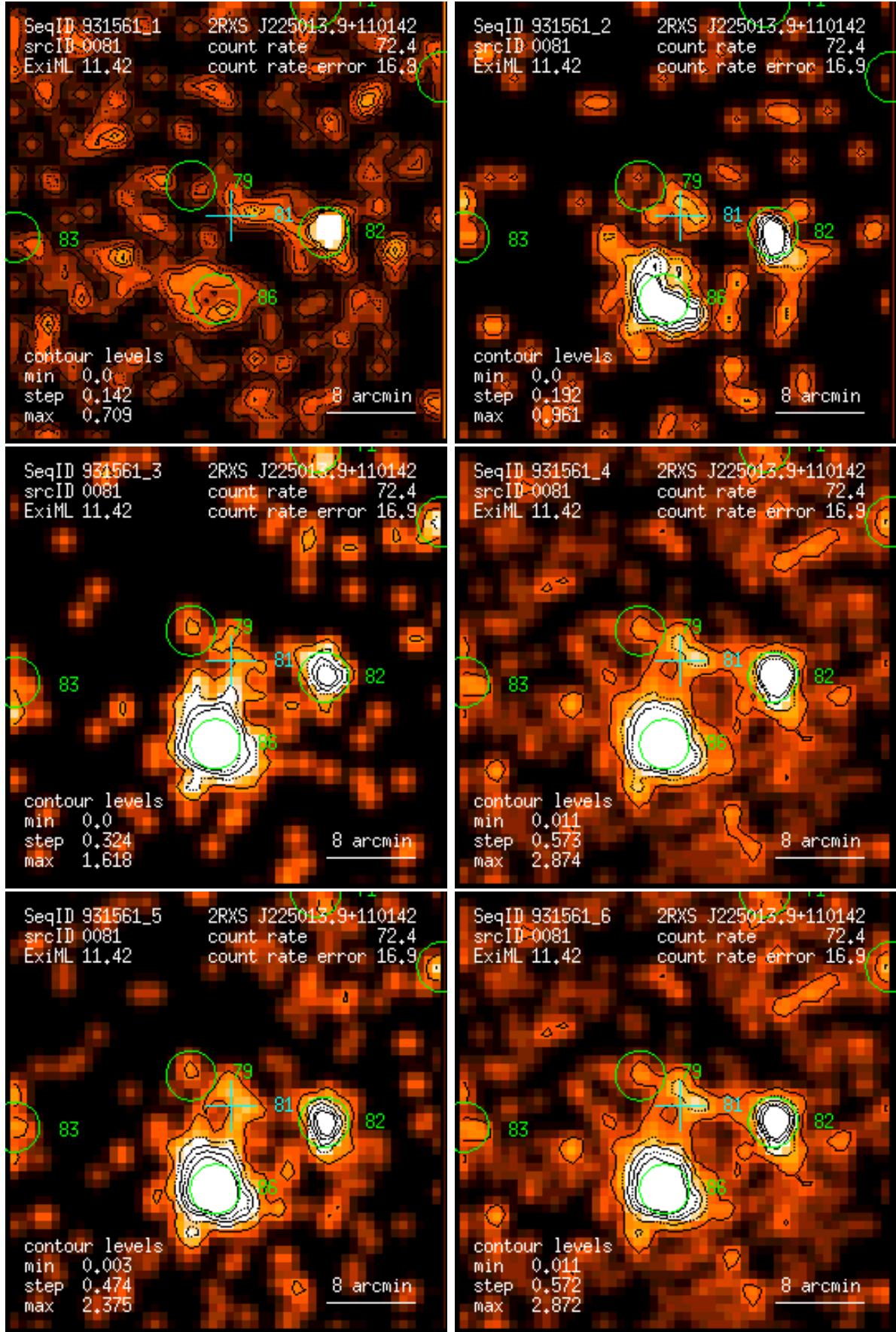
Figure 81: RASS 931561: detection 0081: band rate images, Gaussian filter: (1) PSPC channels 11 – 41, (2) 52 – 90, (3) 91 – 201, (4) 11 – 235, (5) 52 – 201, (6) 11 – 201. Broad band rates in counts/ks. Band rate contour levels in counts/ks/arcmin 2 .
