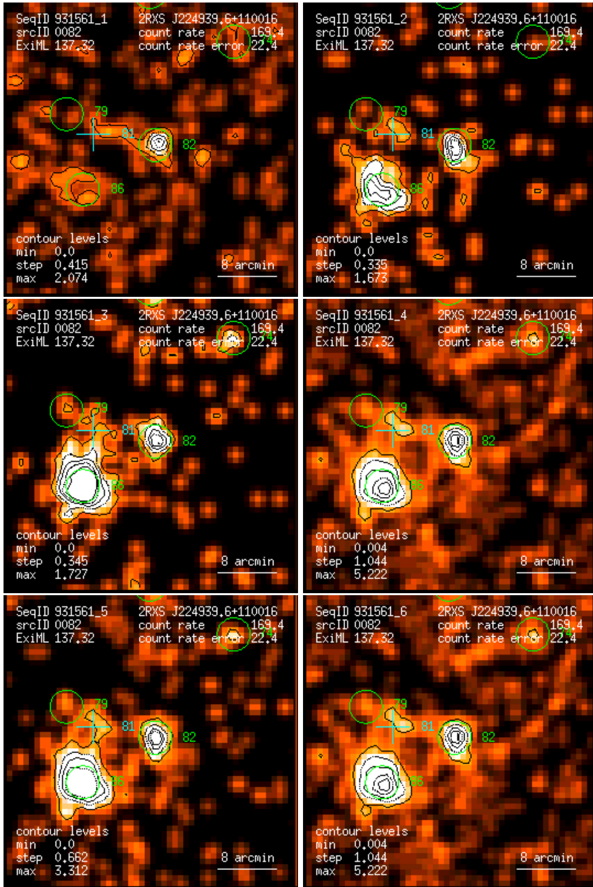
Figure 82: RASS 931561: detection 0082: band rate images, Gaussian filter: (1) PSPC channels 11 – 41, (2) 52 – 90, (3) 91 – 201, (4) 11 – 235, (5) 52 – 201, (6) 11 – 201. Broad band rates in counts/ks. Band rate contour levels in counts/ks/arcmin 2 .
