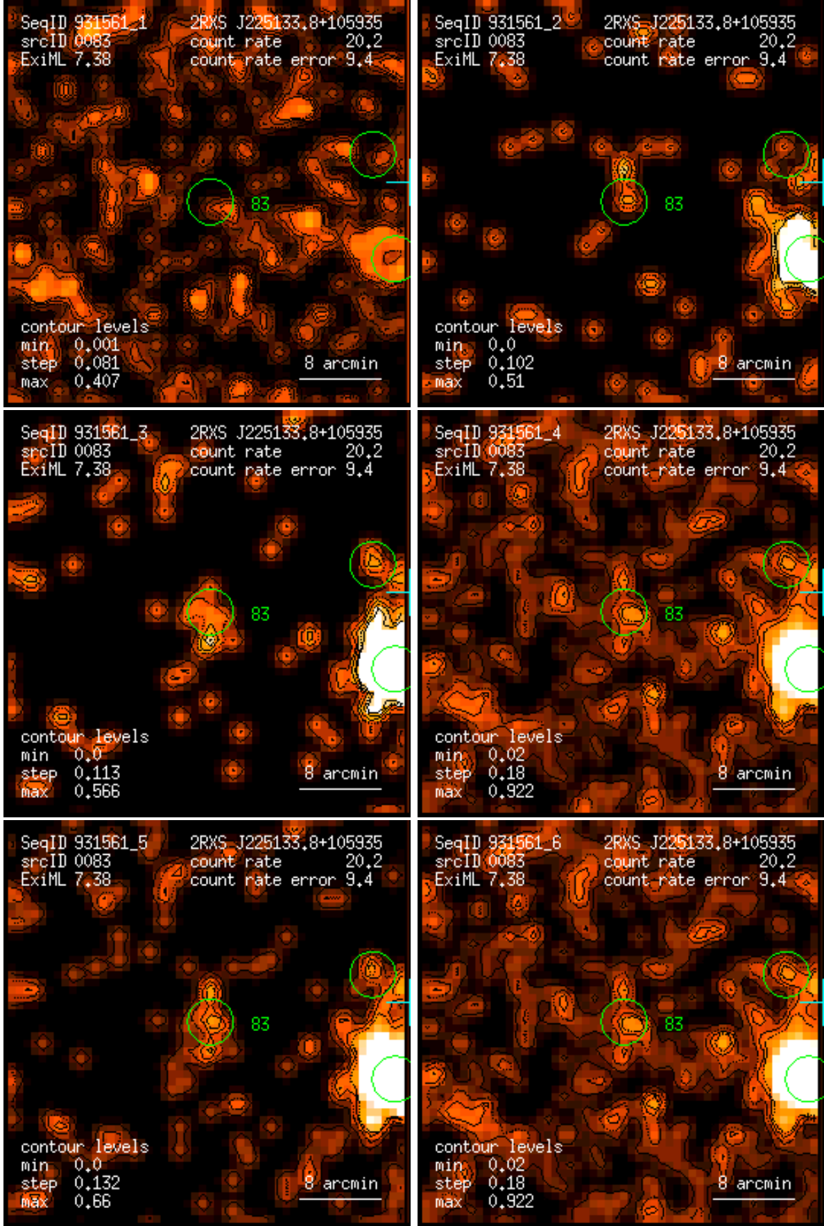
Figure 83: RASS 931561: detection 0083: band rate images, Gaussian filter: (1) PSPC channels 11 – 41, (2) 52 – 90, (3) 91 – 201, (4) 11 – 235, (5) 52 – 201, (6) 11 – 201. Broad band rates in counts/ks. Band rate contour levels in counts/ks/arcmin 2 .
