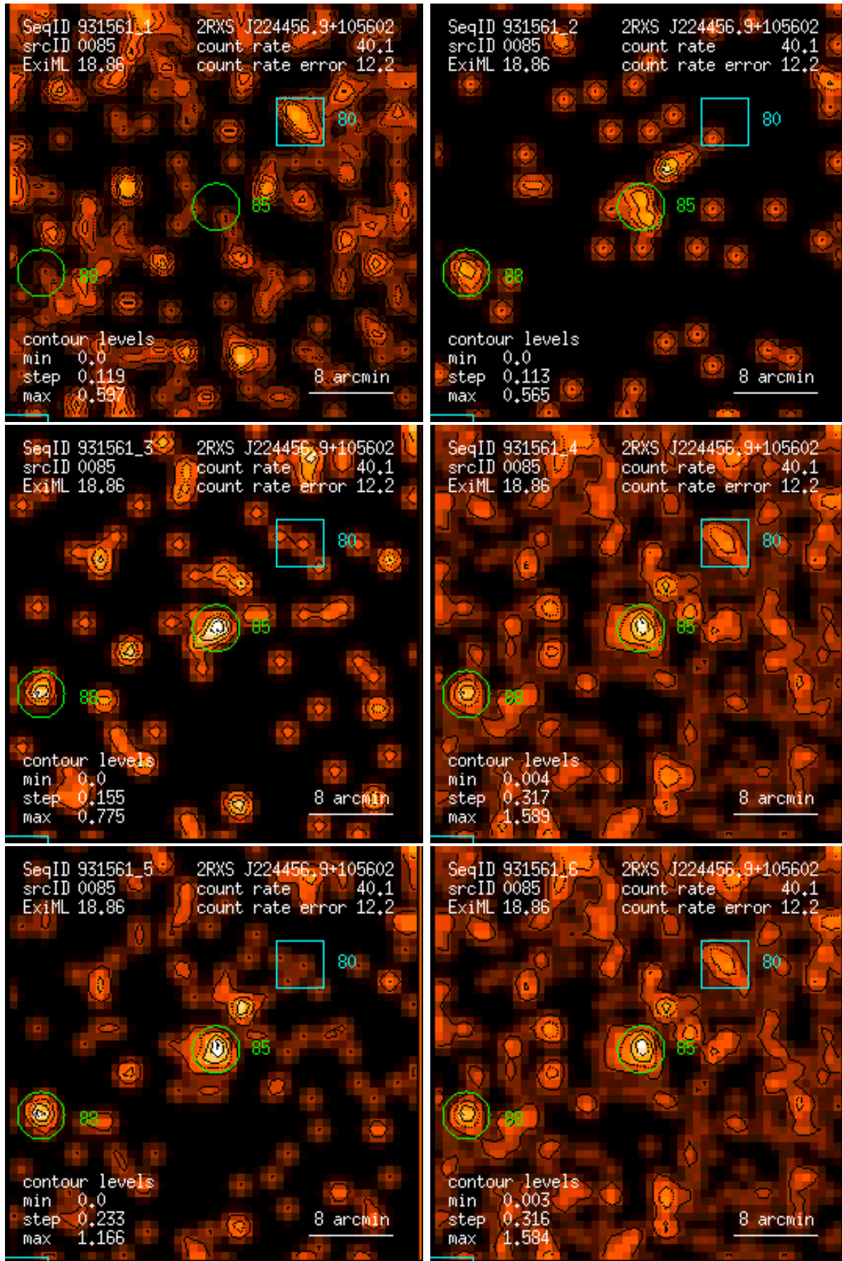
Figure 85: RASS 931561: detection 0085: band rate images, Gaussian filter: (1) PSPC channels 11 – 41, (2) 52 – 90, (3) 91 – 201, (4) 11 – 235, (5) 52 – 201, (6) 11 – 201. Broad band rates in counts/ks. Band rate contour levels in counts/ks/arcmin 2 .
