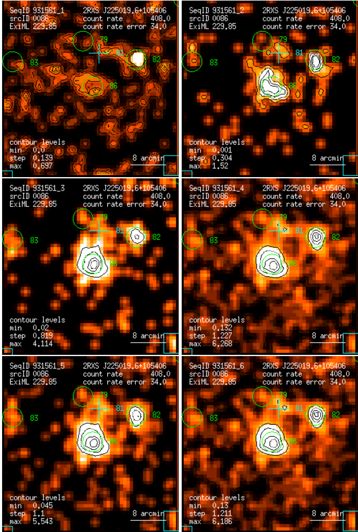
Figure 86: RASS 931561: detection 0086: band rate images, Gaussian filter: (1) PSPC channels 11 – 41, (2) 52 – 90, (3) 91 – 201, (4) 11 – 235, (5) 52 – 201, (6) 11 – 201. Broad band rates in counts/ks. Band rate contour levels in counts/ks/arcmin 2 .
