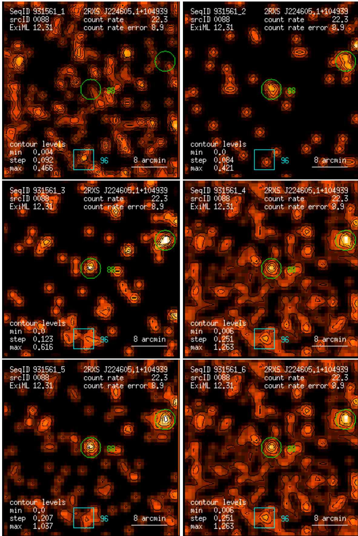
Figure 88: RASS 931561: detection 0088: band rate images, Gaussian filter: (1) PSPC channels 11 – 41, (2) 52 – 90, (3) 91 – 201, (4) 11 – 235, (5) 52 – 201, (6) 11 – 201. Broad band rates in counts/ks. Band rate contour levels in counts/ks/arcmin 2 .
