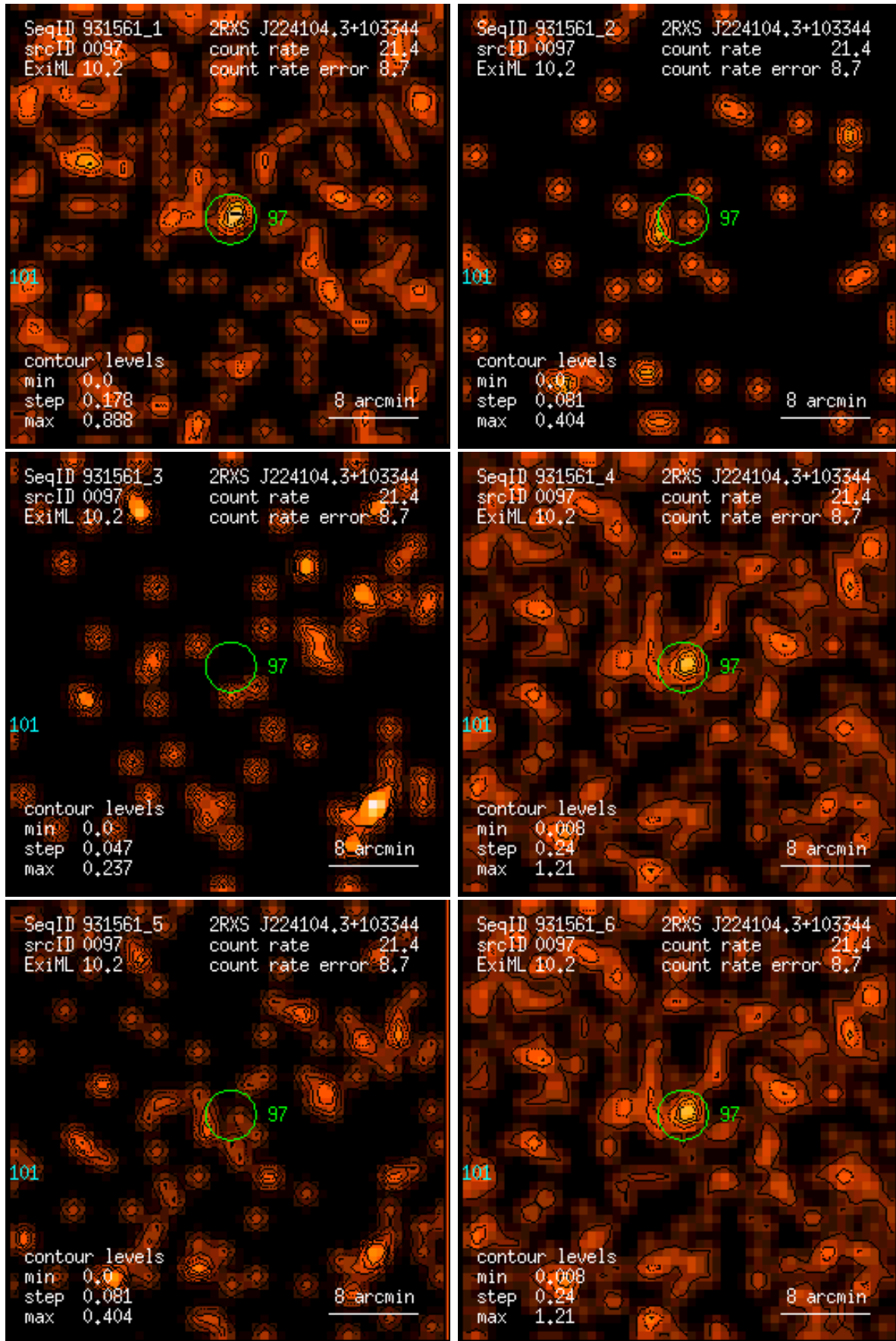
Figure 97: RASS 931561: detection 0097: band rate images, Gaussian filter: (1) PSPC channels 11 – 41, (2) 52 – 90, (3) 91 – 201, (4) 11 – 235, (5) 52 – 201, (6) 11 – 201. Broad band rates in counts/ks. Band rate contour levels in counts/ks/arcmin 2 .
