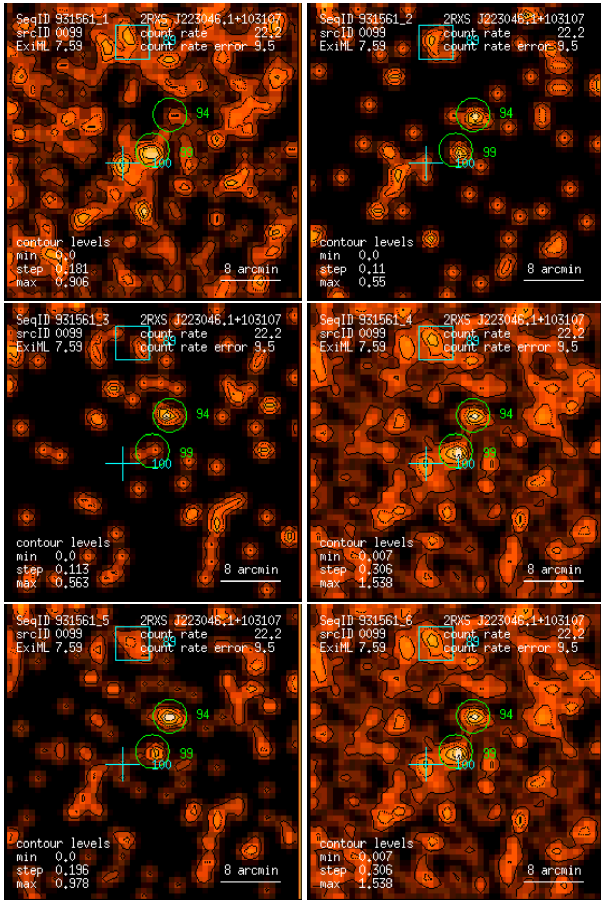
Figure 99: RASS 931561: detection 0099: band rate images, Gaussian filter: (1) PSPC channels 11 – 41, (2) 52 – 90, (3) 91 – 201, (4) 11 – 235, (5) 52 – 201, (6) 11 – 201. Broad band rates in counts/ks. Band rate contour levels in counts/ks/arcmin 2 .
