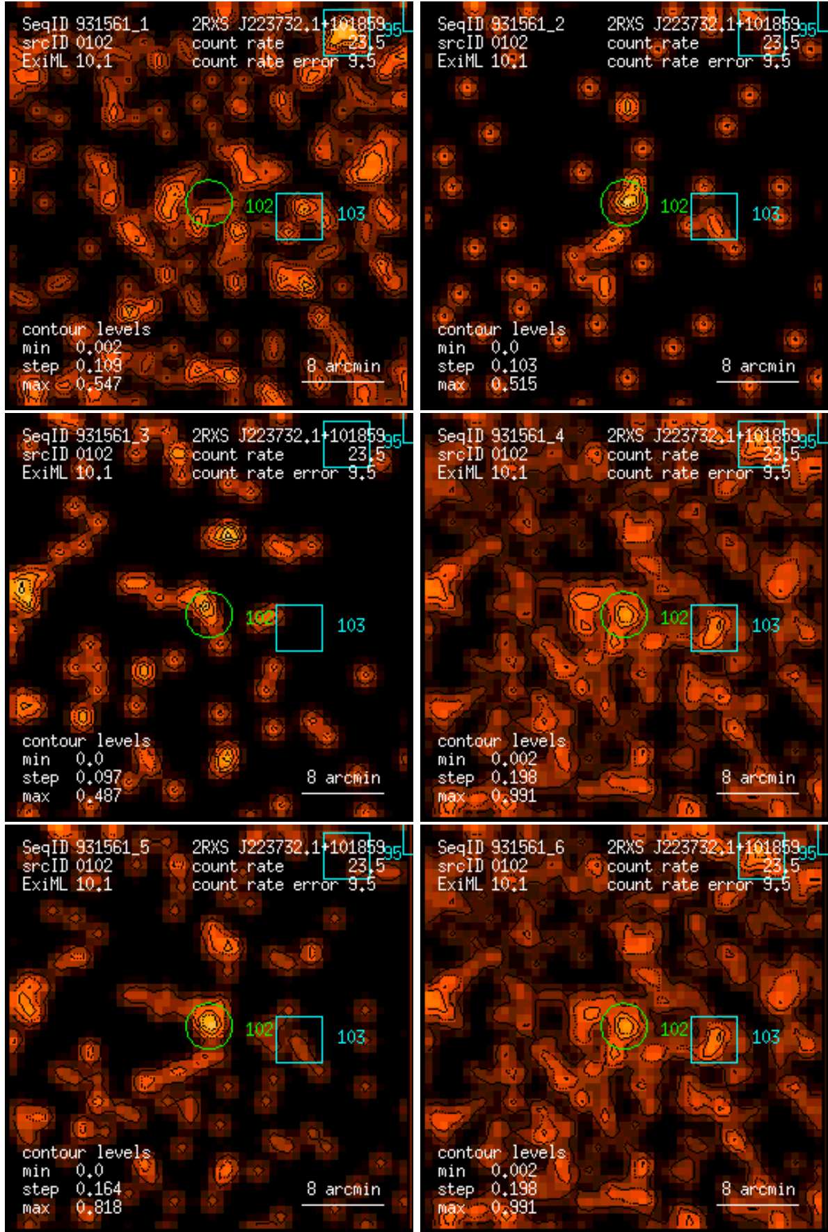
Figure 102: RASS 931561: detection 0102: band rate images, Gaussian filter: (1) PSPC channels 11 – 41, (2) 52 – 90, (3) 91 – 201, (4) 11 – 235, (5) 52 – 201, (6) 11 – 201. Broad band rates in counts/ks. Band rate contour levels in counts/ks/arcmin 2 .
