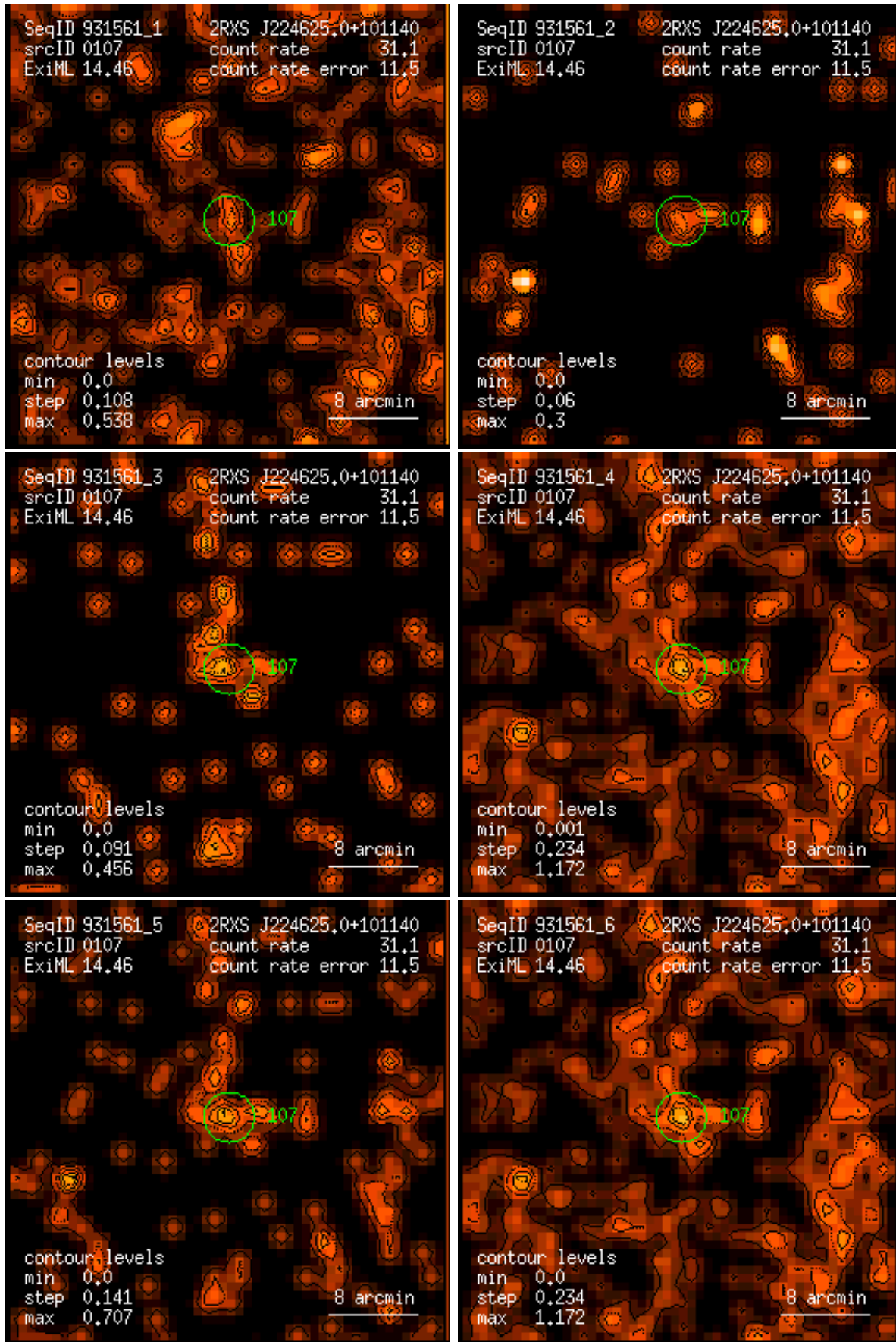
Figure 107: RASS 931561: detection 0107: band rate images, Gaussian filter: (1) PSPC channels 11 – 41, (2) 52 – 90, (3) 91 – 201, (4) 11 – 235, (5) 52 – 201, (6) 11 – 201. Broad band rates in counts/ks. Band rate contour levels in counts/ks/arcmin 2 .
