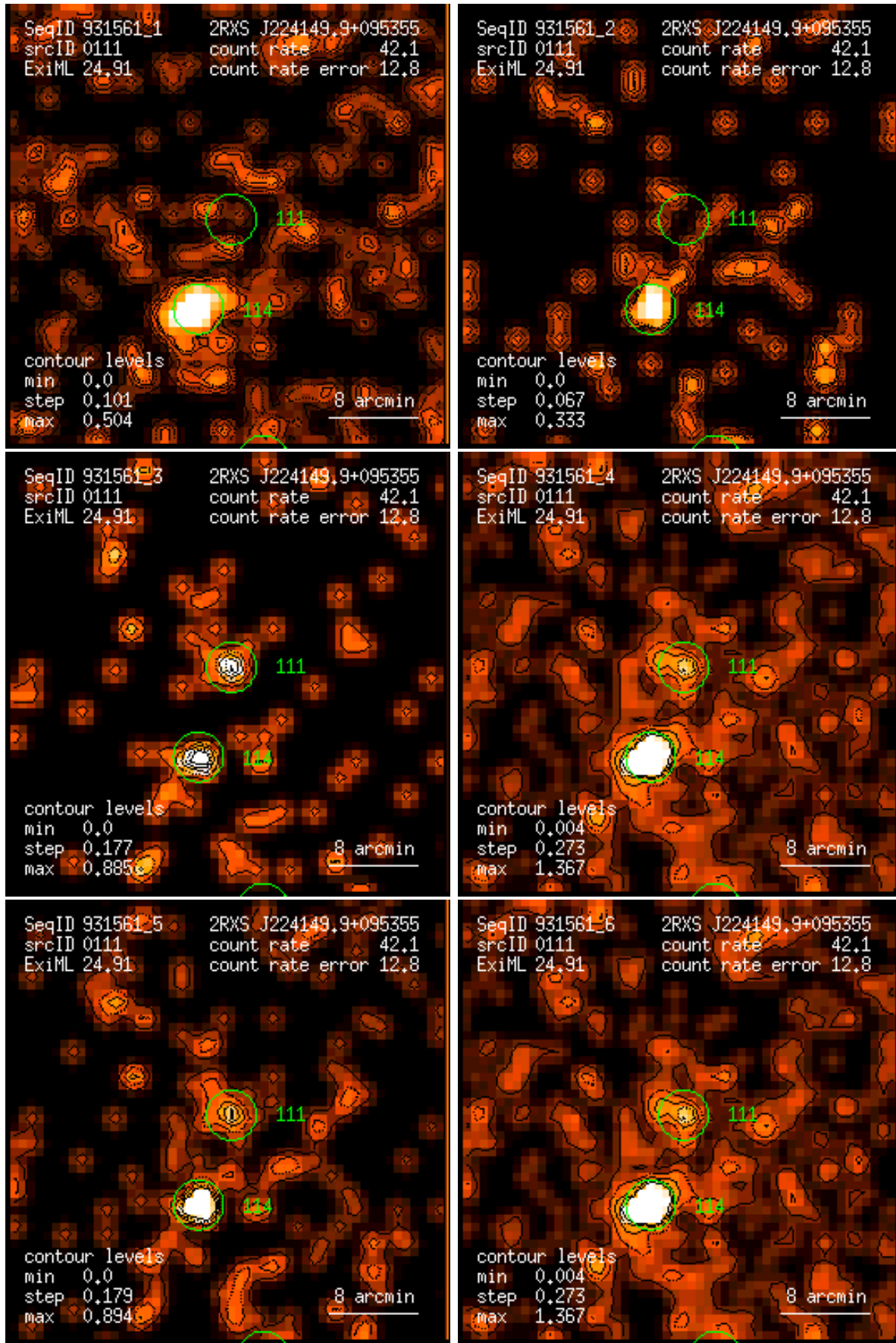
Figure 111: RASS 931561: detection 0111: band rate images, Gaussian filter: (1) PSPC channels 11 – 41, (2) 52 – 90, (3) 91 – 201, (4) 11 – 235, (5) 52 – 201, (6) 11 – 201. Broad band rates in counts/ks. Band rate contour levels in counts/ks/arcmin 2 .
