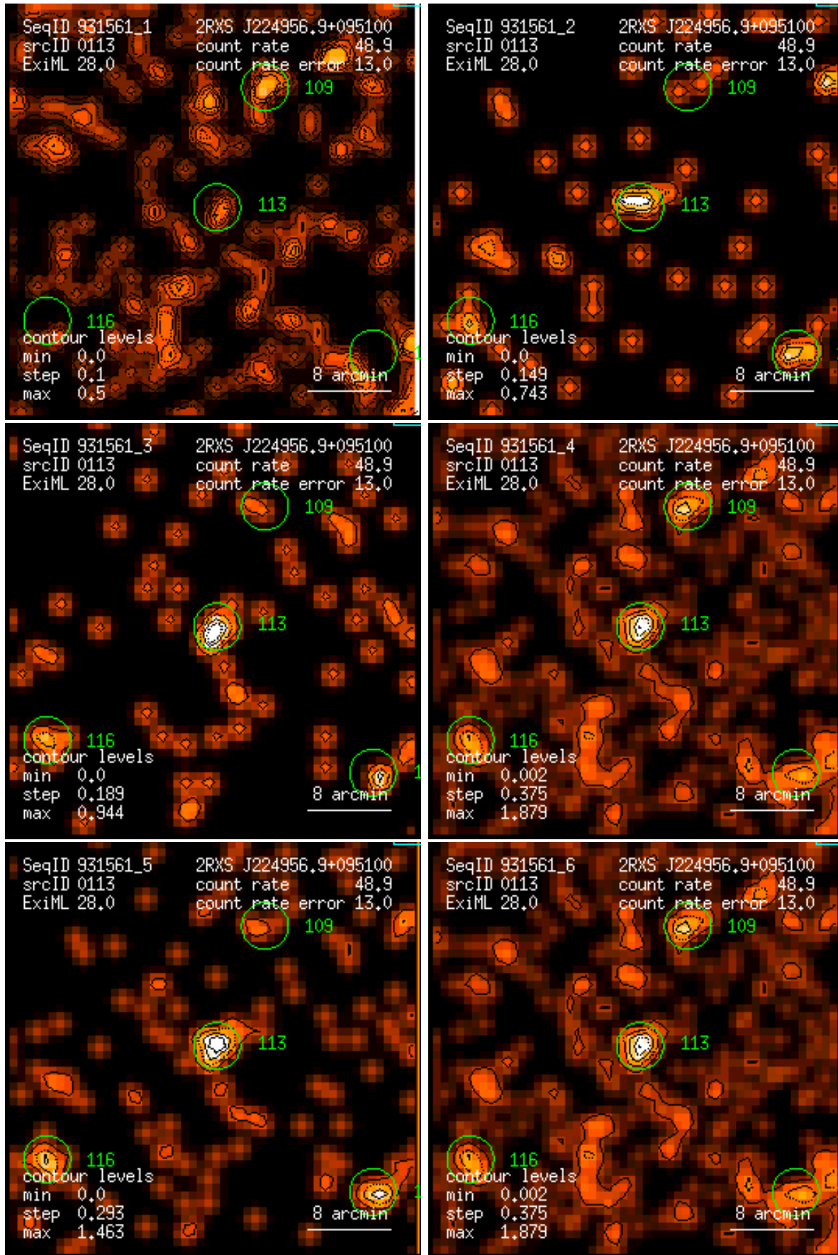
Figure 113: RASS 931561: detection 0113: band rate images, Gaussian filter: (1) PSPC channels 11 – 41, (2) 52 – 90, (3) 91 – 201, (4) 11 – 235, (5) 52 – 201, (6) 11 – 201. Broad band rates in counts/ks. Band rate contour levels in counts/ks/arcmin 2 .
