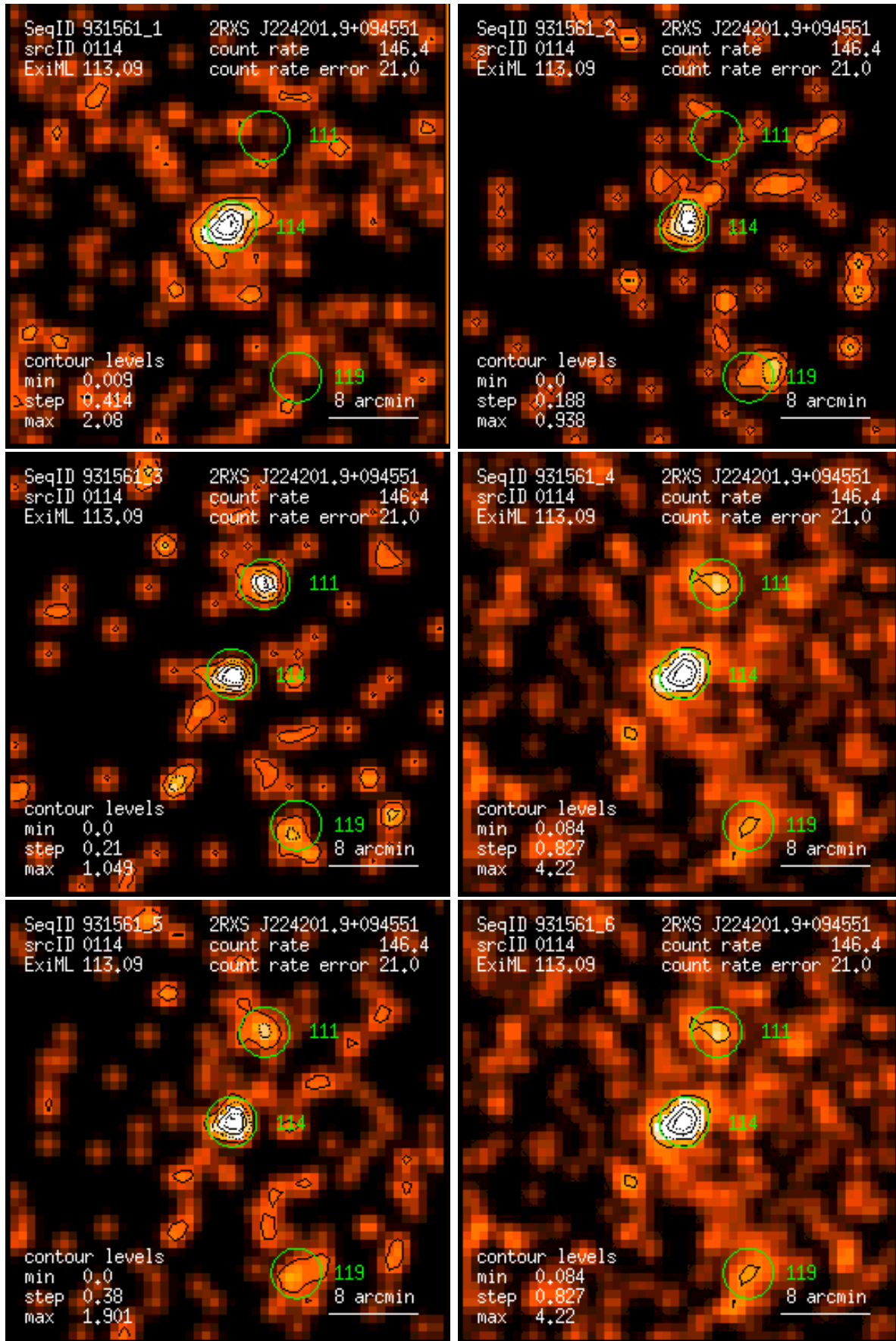
Figure 114: RASS 931561: detection 0114: band rate images, Gaussian filter: (1) PSPC channels 11 – 41, (2) 52 – 90, (3) 91 – 201, (4) 11 – 235, (5) 52 – 201, (6) 11 – 201. Broad band rates in counts/ks. Band rate contour levels in counts/ks/arcmin 2 .
