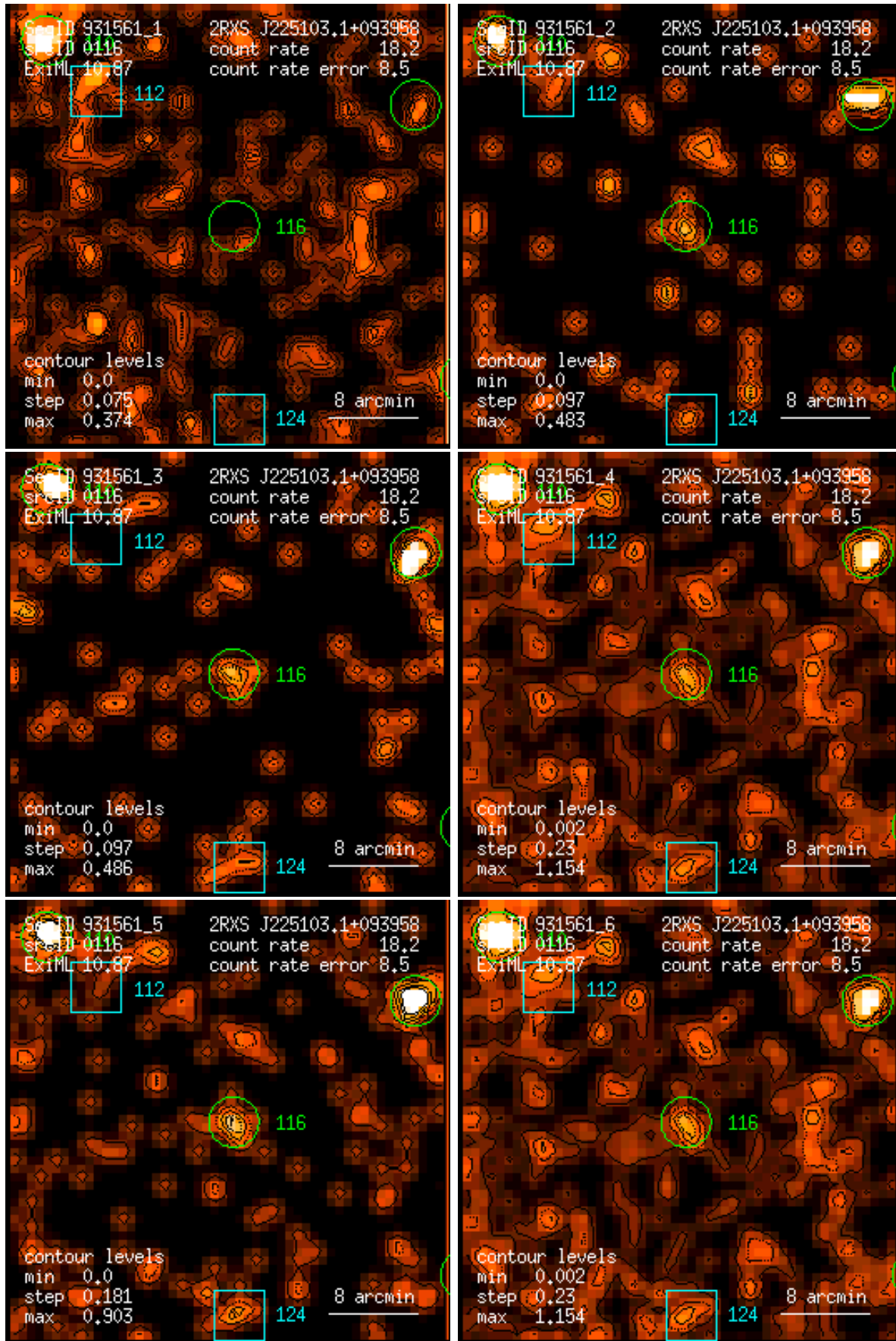
Figure 116: RASS 931561: detection 0116: band rate images, Gaussian filter: (1) PSPC channels 11 – 41, (2) 52 – 90, (3) 91 – 201, (4) 11 – 235, (5) 52 – 201, (6) 11 – 201. Broad band rates in counts/ks. Band rate contour levels in counts/ks/arcmin 2 .
