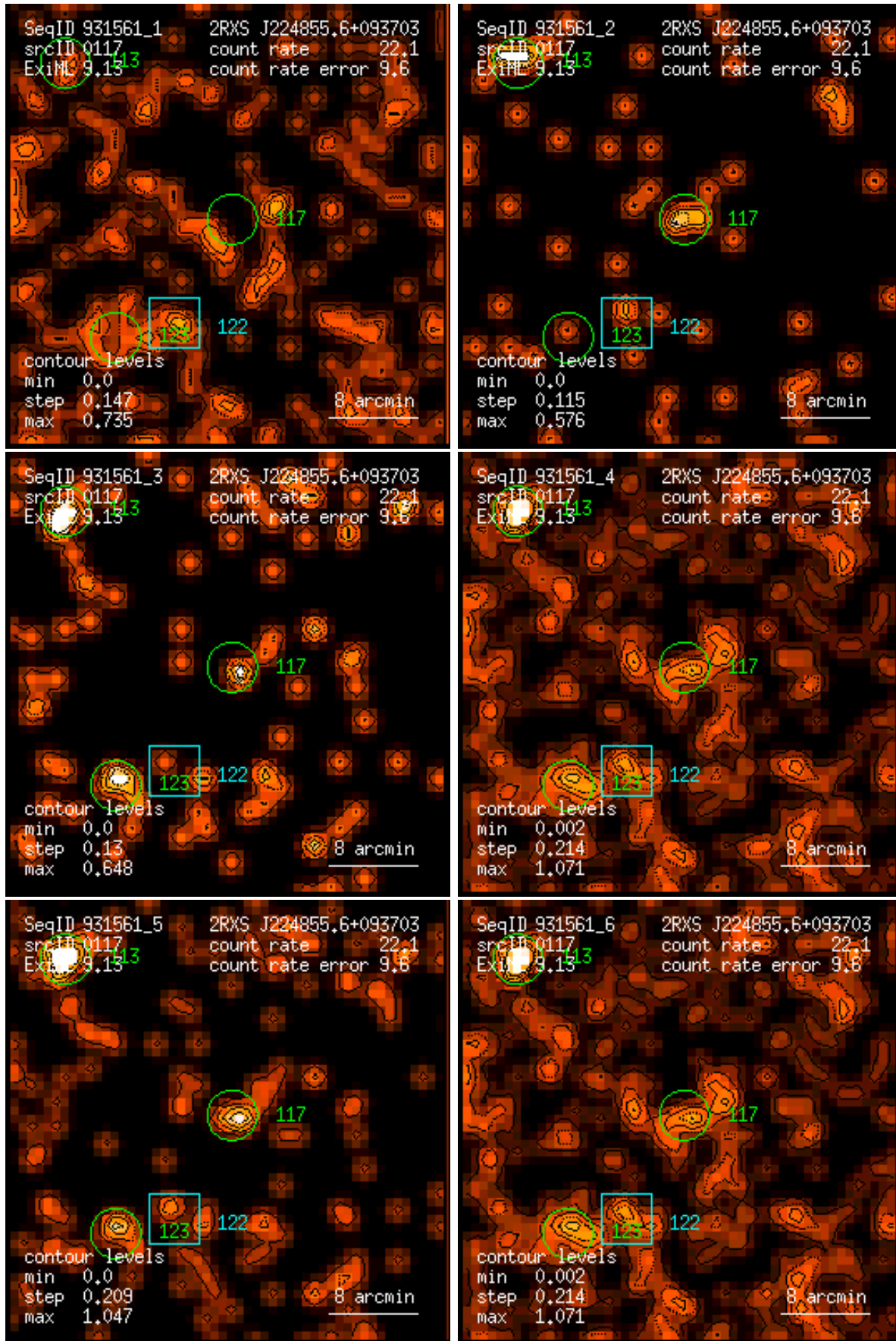
Figure 117: RASS 931561: detection 0117: band rate images, Gaussian filter: (1) PSPC channels 11 – 41, (2) 52 – 90, (3) 91 – 201, (4) 11 – 235, (5) 52 – 201, (6) 11 – 201. Broad band rates in counts/ks. Band rate contour levels in counts/ks/arcmin 2 .
