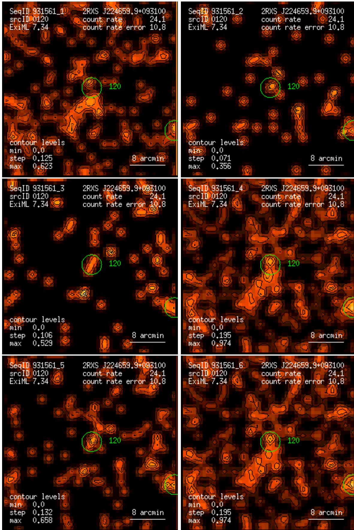
Figure 120: RASS 931561: detection 0120: band rate images, Gaussian filter: (1) PSPC channels 11 – 41, (2) 52 – 90, (3) 91 – 201, (4) 11 – 235, (5) 52 – 201, (6) 11 – 201. Broad band rates in counts/ks. Band rate contour levels in counts/ks/arcmin 2 .
