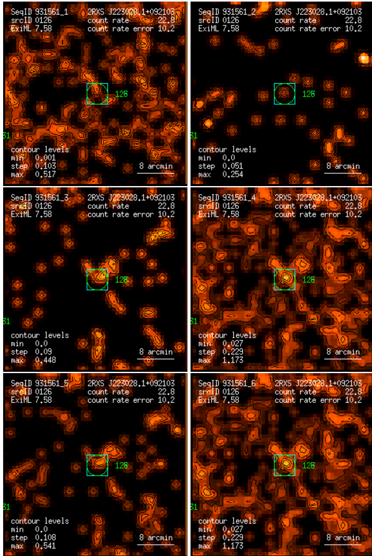
Figure 126: RASS 931561: detection 0126: band rate images, Gaussian filter: (1) PSPC channels 11 – 41, (2) 52 – 90, (3) 91 – 201, (4) 11 – 235, (5) 52 – 201, (6) 11 – 201. Broad band rates in counts/ks. Band rate contour levels in counts/ks/arcmin 2 .
