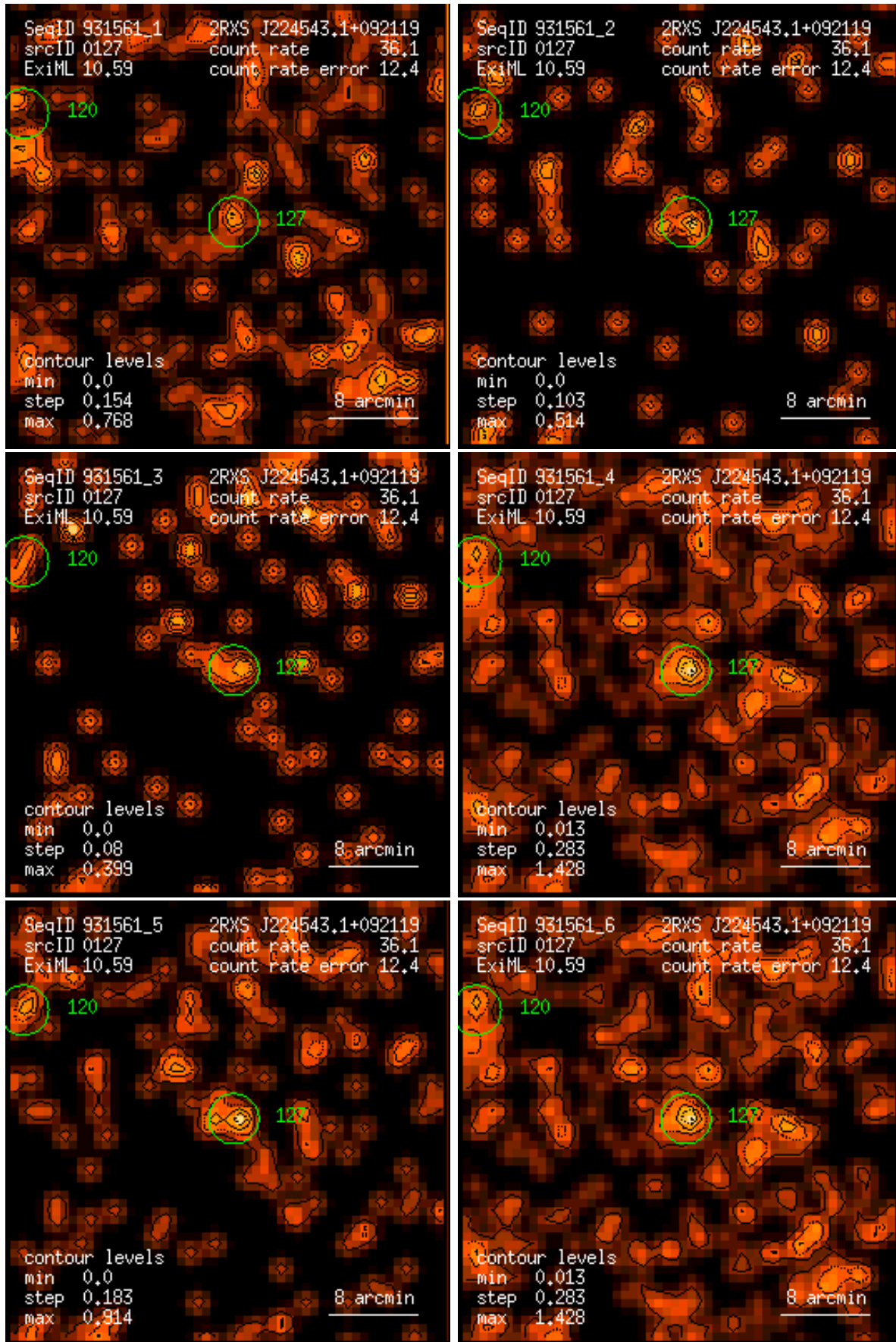
Figure 127: RASS 931561: detection 0127: band rate images, Gaussian filter: (1) PSPC channels 11 – 41, (2) 52 – 90, (3) 91 – 201, (4) 11 – 235, (5) 52 – 201, (6) 11 – 201. Broad band rates in counts/ks. Band rate contour levels in counts/ks/arcmin 2 .
