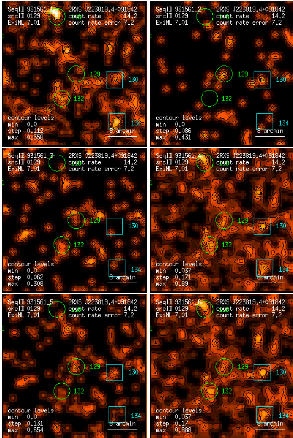
Figure 129: RASS 931561: detection 0129: band rate images, Gaussian filter: (1) PSPC channels 11 – 41, (2) 52 – 90, (3) 91 – 201, (4) 11 – 235, (5) 52 – 201, (6) 11 – 201. Broad band rates in counts/ks. Band rate contour levels in counts/ks/arcmin 2 .
