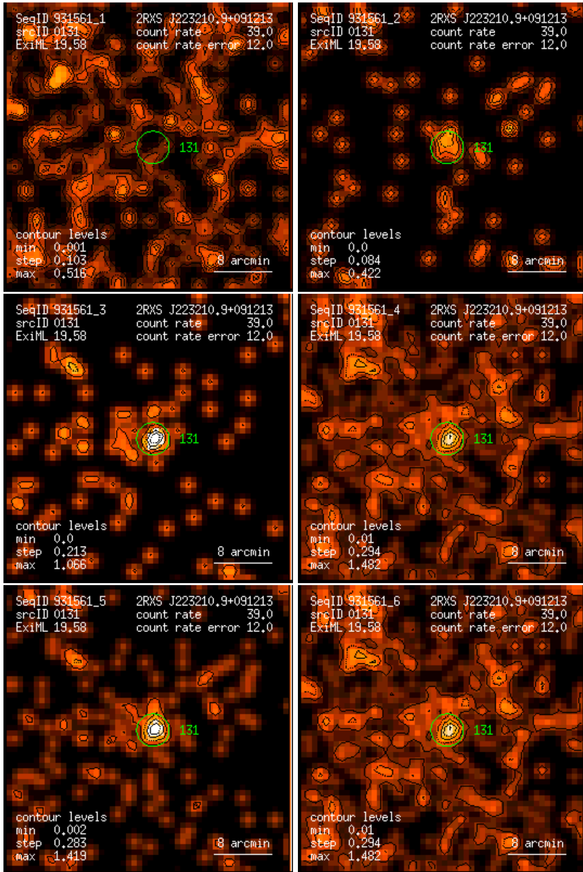
Figure 131: RASS 931561: detection 0131: band rate images, Gaussian filter: (1) PSPC channels 11 – 41, (2) 52 – 90, (3) 91 – 201, (4) 11 – 235, (5) 52 – 201, (6) 11 – 201. Broad band rates in counts/ks. Band rate contour levels in counts/ks/arcmin 2 .
