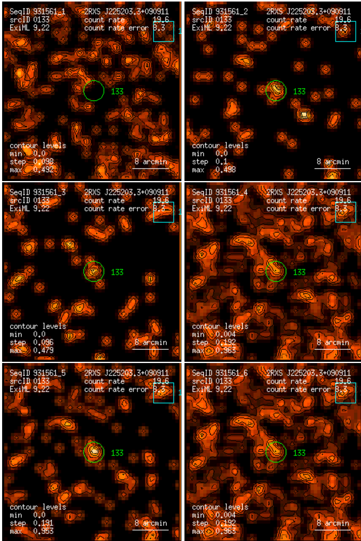
Figure 133: RASS 931561: detection 0133: band rate images, Gaussian filter: (1) PSPC channels 11 – 41, (2) 52 – 90, (3) 91 – 201, (4) 11 – 235, (5) 52 – 201, (6) 11 – 201. Broad band rates in counts/ks. Band rate contour levels in counts/ks/arcmin 2 .
