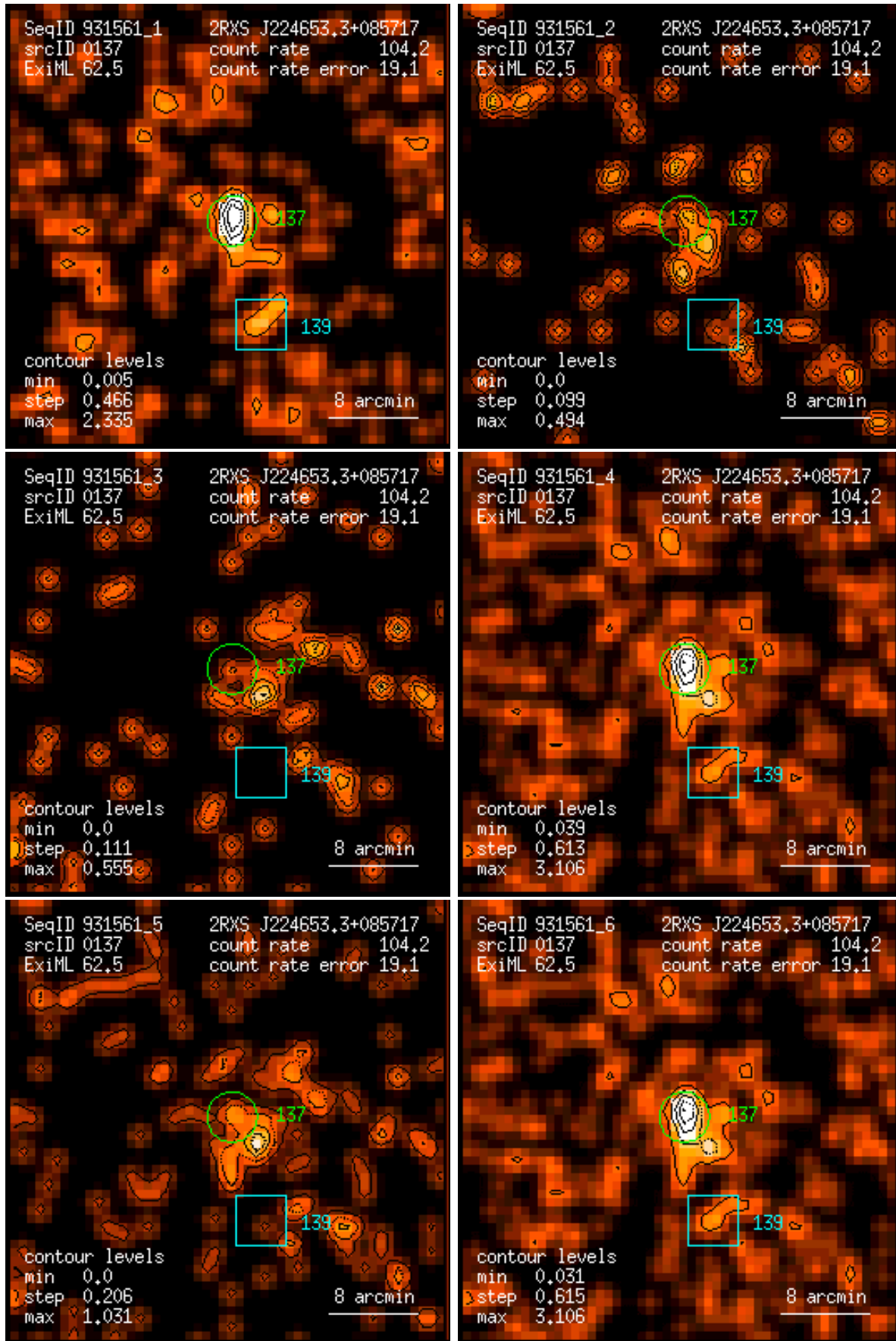
Figure 137: RASS 931561: detection 0137: band rate images, Gaussian filter: (1) PSPC channels 11 – 41, (2) 52 – 90, (3) 91 – 201, (4) 11 – 235, (5) 52 – 201, (6) 11 – 201. Broad band rates in counts/ks. Band rate contour levels in counts/ks/arcmin 2 .
