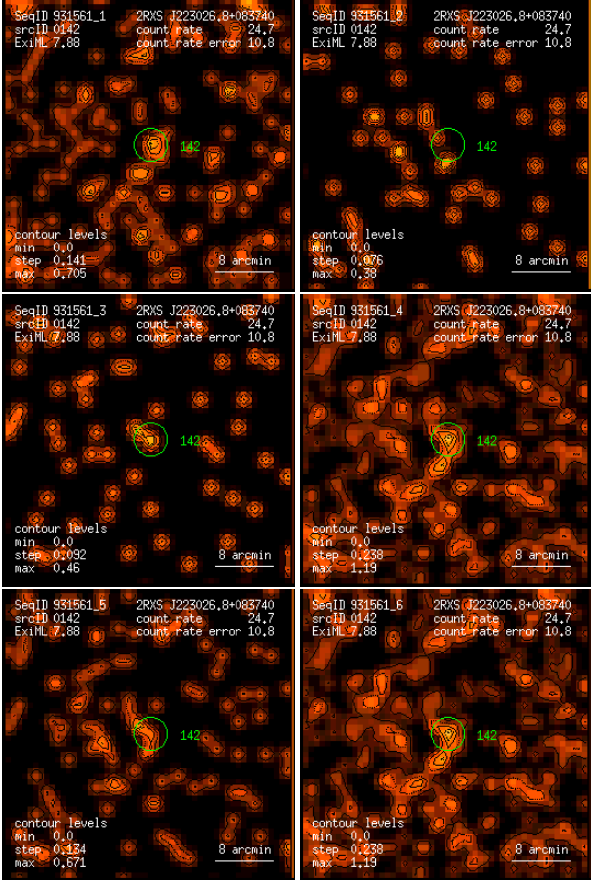
Figure 142: RASS 931561: detection 0142: band rate images, Gaussian filter: (1) PSPC channels 11 – 41, (2) 52 – 90, (3) 91 – 201, (4) 11 – 235, (5) 52 – 201, (6) 11 – 201. Broad band rates in counts/ks. Band rate contour levels in counts/ks/arcmin 2 .
