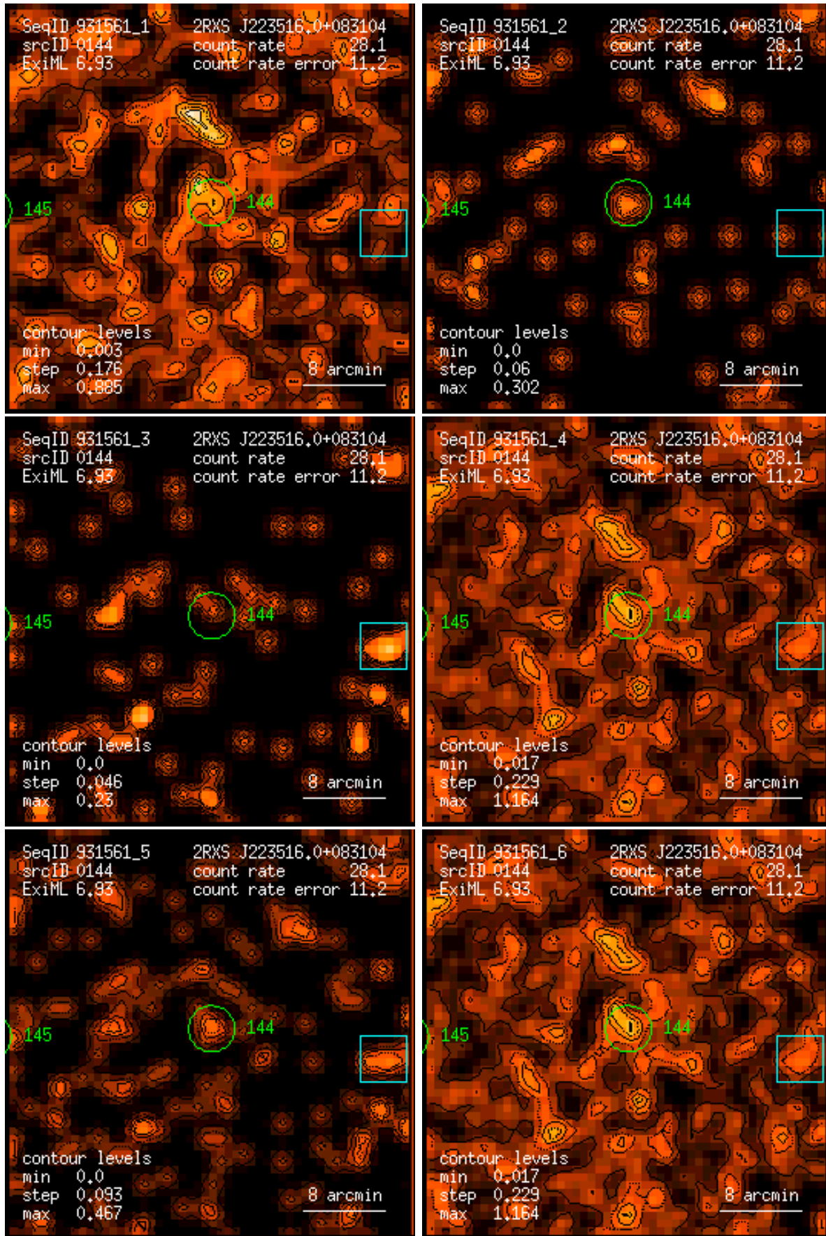
Figure 144: RASS 931561: detection 0144: band rate images, Gaussian filter: (1) PSPC channels 11 – 41, (2) 52 – 90, (3) 91 – 201, (4) 11 – 235, (5) 52 – 201, (6) 11 – 201. Broad band rates in counts/ks. Band rate contour levels in counts/ks/arcmin 2 .
