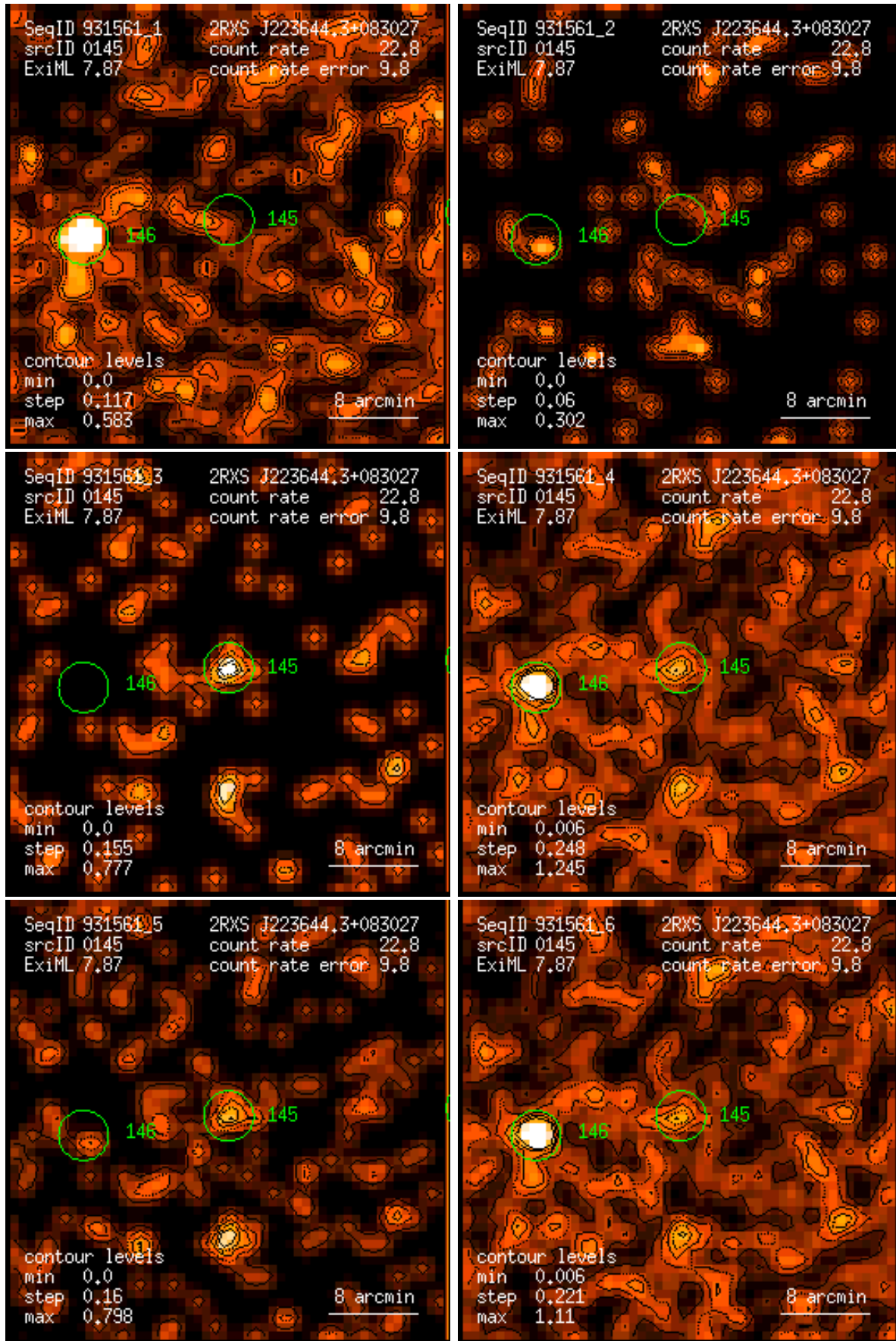
Figure 145: RASS 931561: detection 0145: band rate images, Gaussian filter: (1) PSPC channels 11 – 41, (2) 52 – 90, (3) 91 – 201, (4) 11 – 235, (5) 52 – 201, (6) 11 – 201. Broad band rates in counts/ks. Band rate contour levels in counts/ks/arcmin 2 .
