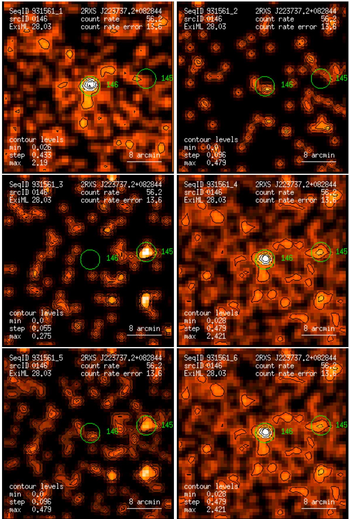
Figure 146: RASS 931561: detection 0146: band rate images, Gaussian filter: (1) PSPC channels 11 – 41, (2) 52 – 90, (3) 91 – 201, (4) 11 – 235, (5) 52 – 201, (6) 11 – 201. Broad band rates in counts/ks. Band rate contour levels in counts/ks/arcmin 2 .
