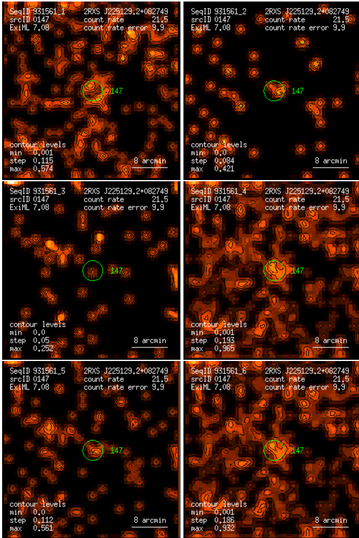
Figure 147: RASS 931561: detection 0147: band rate images, Gaussian filter: (1) PSPC channels 11 – 41, (2) 52 – 90, (3) 91 – 201, (4) 11 – 235, (5) 52 – 201, (6) 11 – 201. Broad band rates in counts/ks. Band rate contour levels in counts/ks/arcmin 2 .
