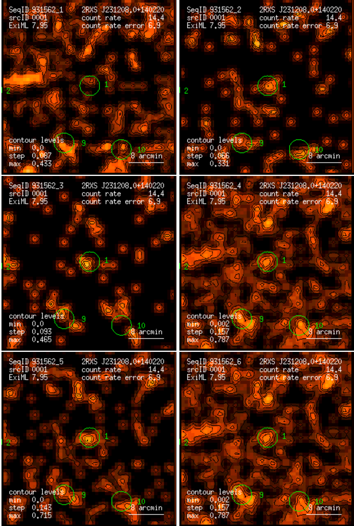
Figure 1: RASS 931562: detection 0001: band rate images, Gaussian filter: (1) PSPC channels 11 – 41, (2) 52 – 90, (3) 91 – 201, (4) 11 – 235, (5) 52 – 201, (6) 11 – 201. Broad band rates in counts/ks. Band rate contour levels in counts/ks/arcmin 2 .
