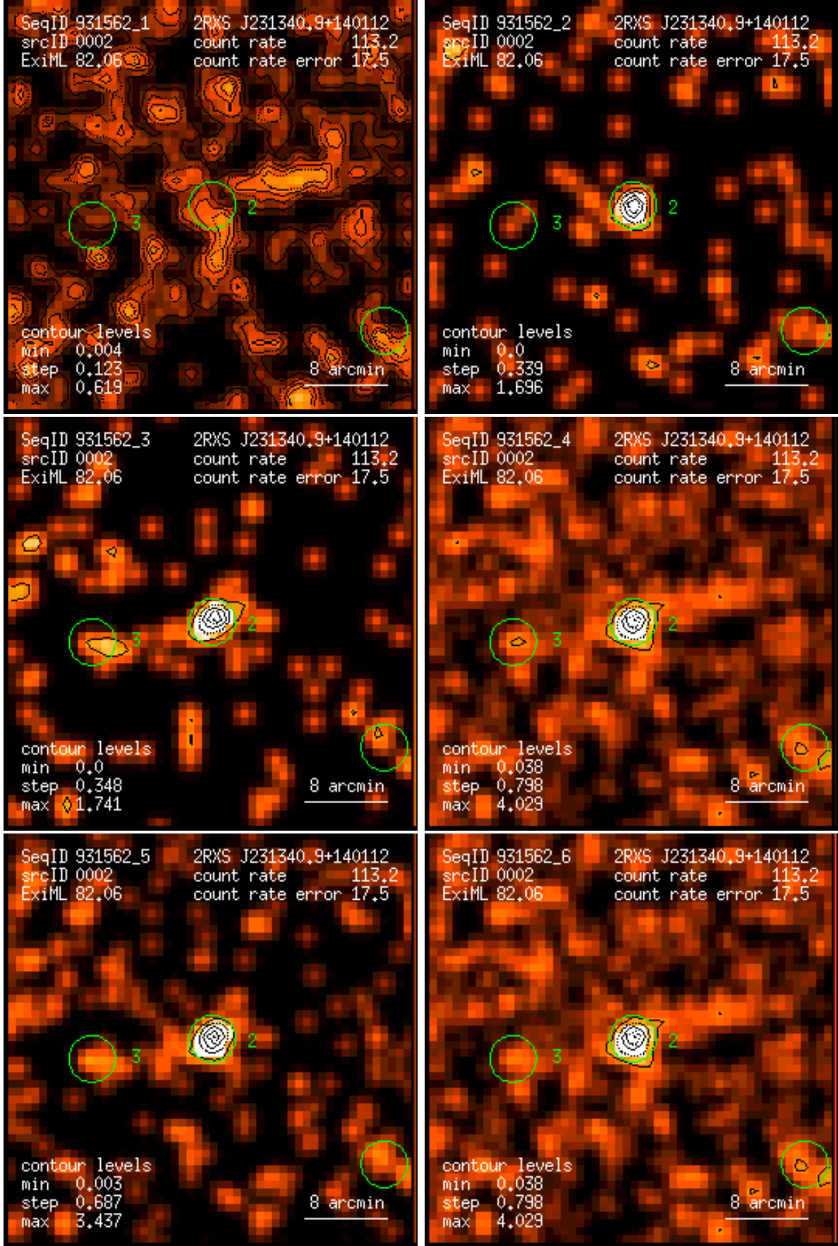
Figure 2: RASS 931562: detection 0002: band rate images, Gaussian filter: (1) PSPC channels 11 – 41, (2) 52 – 90, (3) 91 – 201, (4) 11 – 235, (5) 52 – 201, (6) 11 – 201. Broad band rates in counts/ks. Band rate contour levels in counts/ks/arcmin 2 .
