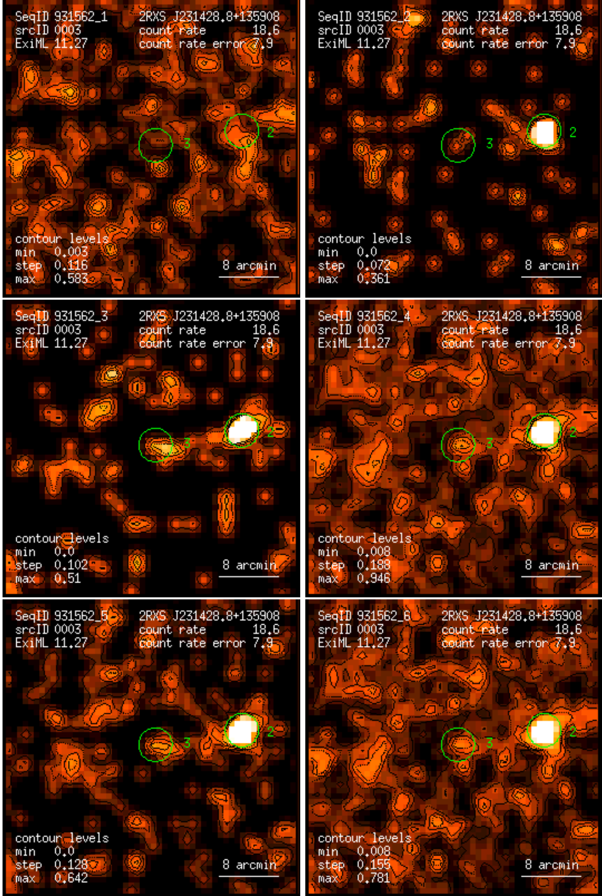
Figure 3: RASS 931562: detection 0003: band rate images, Gaussian filter: (1) PSPC channels 11 – 41, (2) 52 – 90, (3) 91 – 201, (4) 11 – 235, (5) 52 – 201, (6) 11 – 201. Broad band rates in counts/ks. Band rate contour levels in counts/ks/arcmin 2 .
