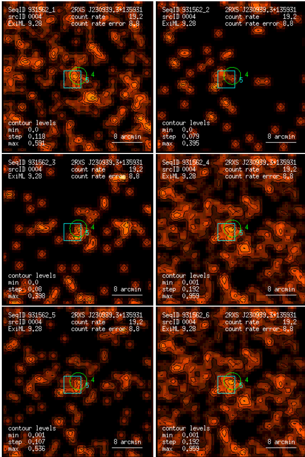
Figure 4: RASS 931562: detection 0004: band rate images, Gaussian filter: (1) PSPC channels 11 – 41, (2) 52 – 90, (3) 91 – 201, (4) 11 – 235, (5) 52 – 201, (6) 11 – 201. Broad band rates in counts/ks. Band rate contour levels in counts/ks/arcmin 2 .
