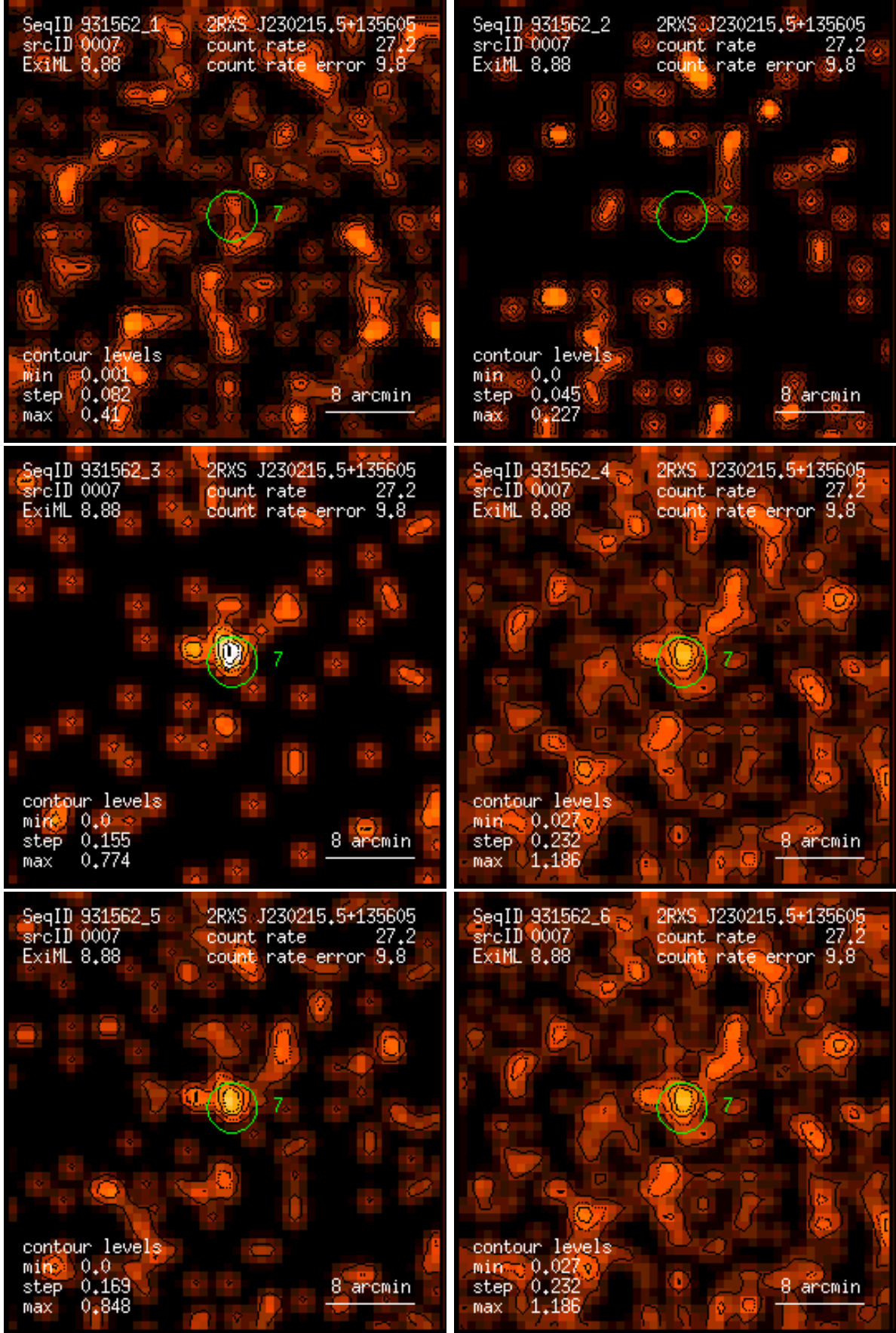
Figure 7: RASS 931562: detection 0007: band rate images, Gaussian filter: (1) PSPC channels 11 – 41, (2) 52 – 90, (3) 91 – 201, (4) 11 – 235, (5) 52 – 201, (6) 11 – 201. Broad band rates in counts/ks. Band rate contour levels in counts/ks/arcmin 2 .
