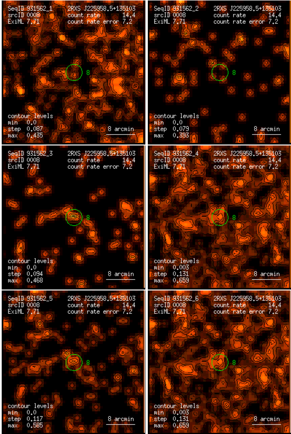
Figure 8: RASS 931562: detection 0008: band rate images, Gaussian filter: (1) PSPC channels 11 – 41, (2) 52 – 90, (3) 91 – 201, (4) 11 – 235, (5) 52 – 201, (6) 11 – 201. Broad band rates in counts/ks. Band rate contour levels in counts/ks/arcmin 2 .
