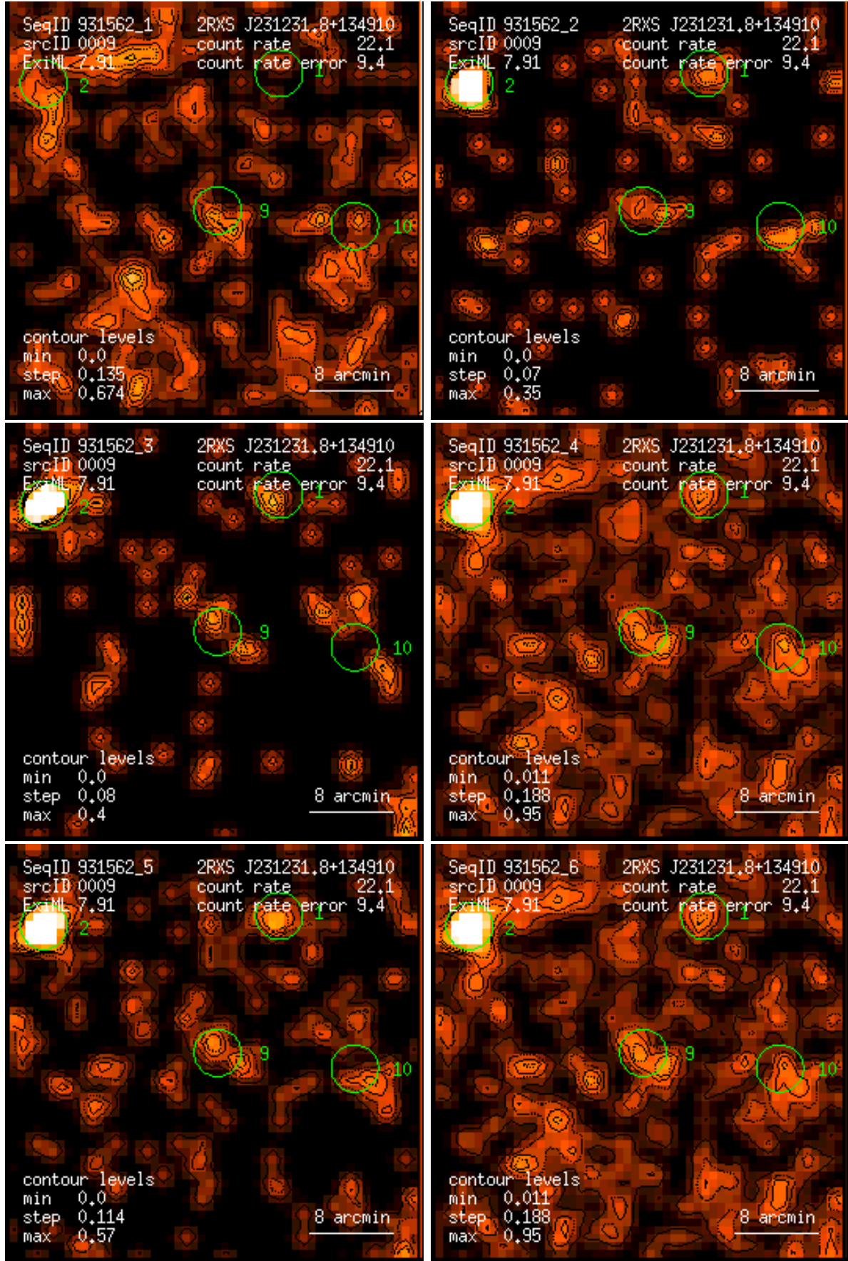
Figure 9: RASS 931562: detection 0009: band rate images, Gaussian filter: (1) PSPC channels 11 – 41, (2) 52 – 90, (3) 91 – 201, (4) 11 – 235, (5) 52 – 201, (6) 11 – 201. Broad band rates in counts/ks. Band rate contour levels in counts/ks/arcmin 2 .
