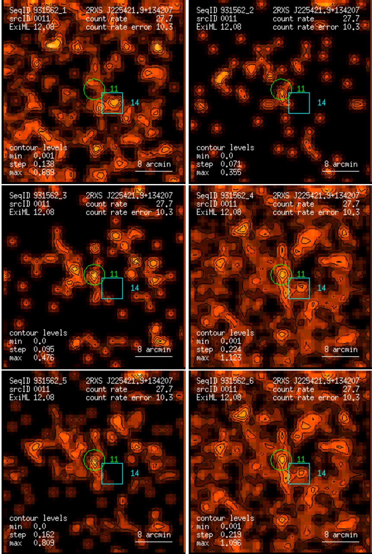
Figure 11: RASS 931562: detection 0011: band rate images, Gaussian filter: (1) PSPC channels 11 – 41, (2) 52 – 90, (3) 91 – 201, (4) 11 – 235, (5) 52 – 201, (6) 11 – 201. Broad band rates in counts/ks. Band rate contour levels in counts/ks/arcmin 2 .
