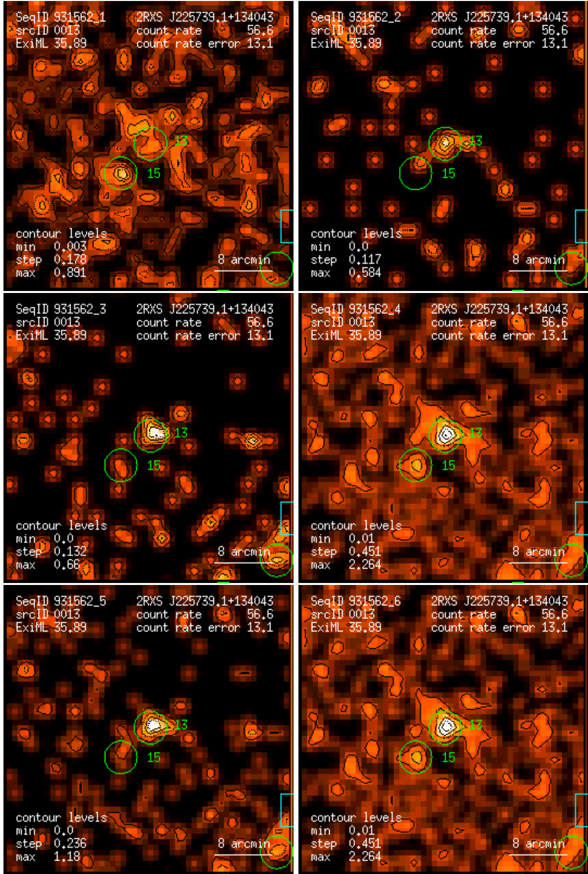
Figure 13: RASS 931562: detection 0013: band rate images, Gaussian filter: (1) PSPC channels 11 – 41, (2) 52 – 90, (3) 91 – 201, (4) 11 – 235, (5) 52 – 201, (6) 11 – 201. Broad band rates in counts/ks. Band rate contour levels in counts/ks/arcmin 2 .
