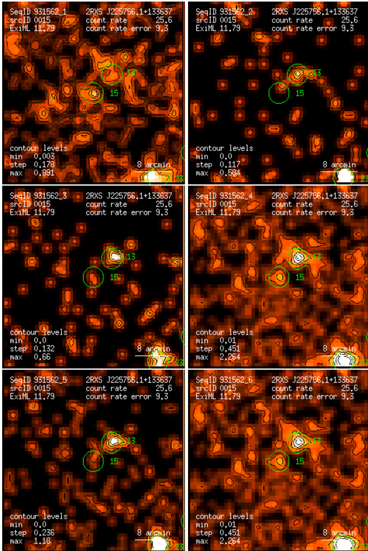
Figure 15: RASS 931562: detection 0015: band rate images, Gaussian filter: (1) PSPC channels 11 – 41, (2) 52 – 90, (3) 91 – 201, (4) 11 – 235, (5) 52 – 201, (6) 11 – 201. Broad band rates in counts/ks. Band rate contour levels in counts/ks/arcmin 2 .
