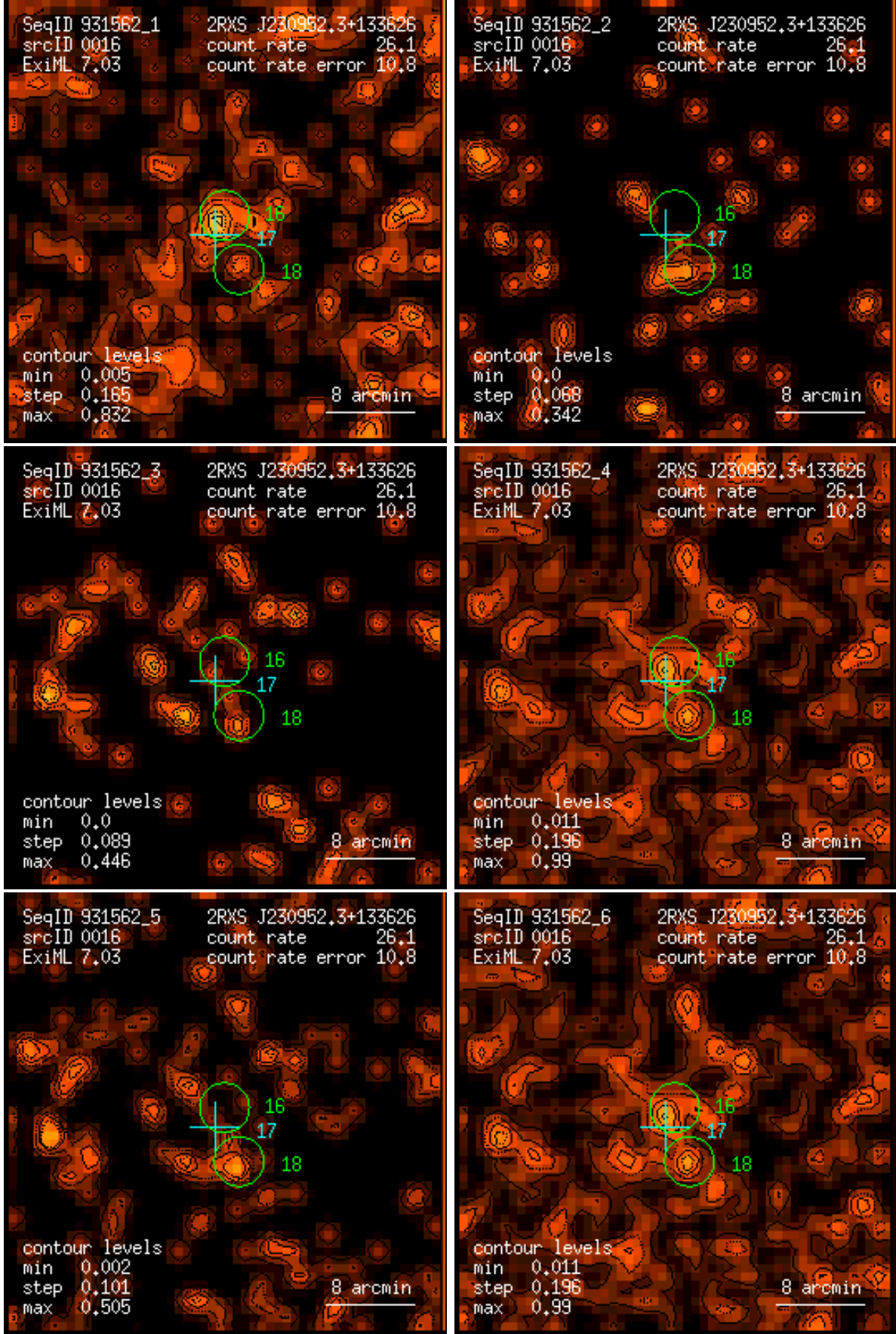
Figure 16: RASS 931562: detection 0016: band rate images, Gaussian filter: (1) PSPC channels 11 – 41, (2) 52 – 90, (3) 91 – 201, (4) 11 – 235, (5) 52 – 201, (6) 11 – 201. Broad band rates in counts/ks. Band rate contour levels in counts/ks/arcmin 2 .
