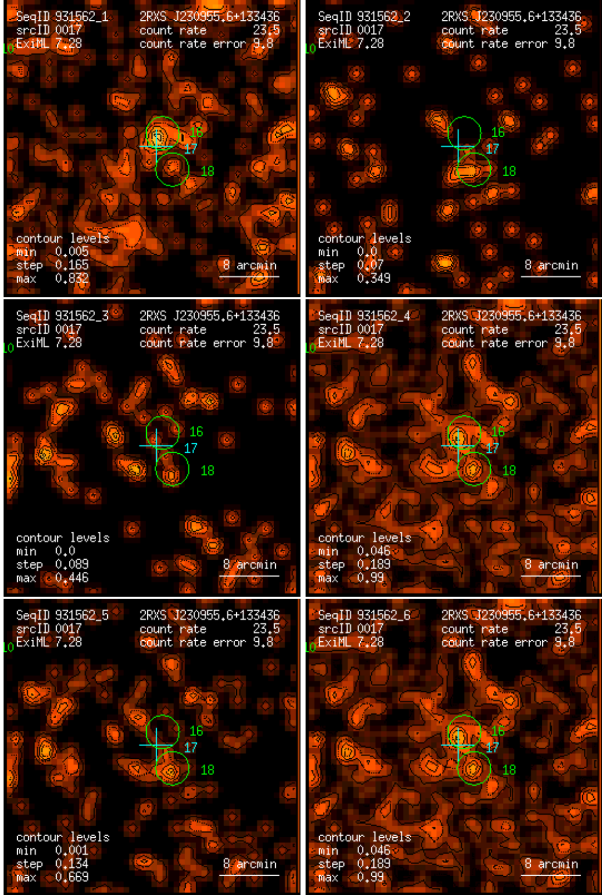
Figure 17: RASS 931562: detection 0017: band rate images, Gaussian filter: (1) PSPC channels 11 – 41, (2) 52 – 90, (3) 91 – 201, (4) 11 – 235, (5) 52 – 201, (6) 11 – 201. Broad band rates in counts/ks. Band rate contour levels in counts/ks/arcmin 2 .
