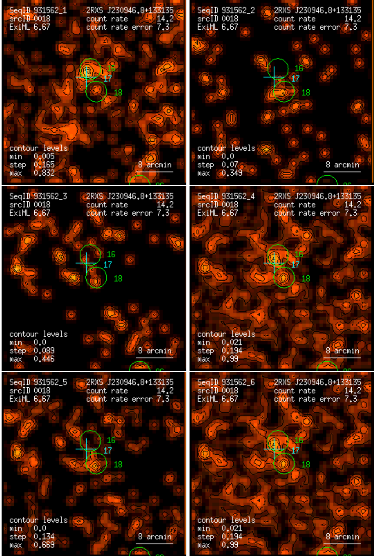
Figure 18: RASS 931562: detection 0018: band rate images, Gaussian filter: (1) PSPC channels 11 – 41, (2) 52 – 90, (3) 91 – 201, (4) 11 – 235, (5) 52 – 201, (6) 11 – 201. Broad band rates in counts/ks. Band rate contour levels in counts/ks/arcmin 2 .
