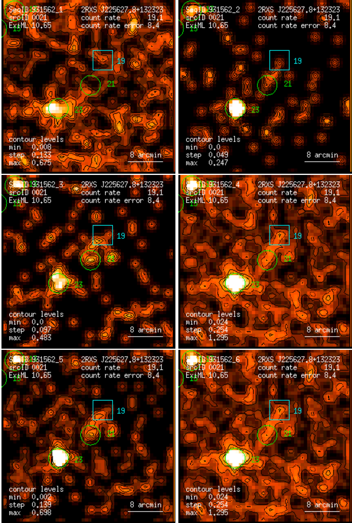
Figure 21: RASS 931562: detection 0021: band rate images, Gaussian filter: (1) PSPC channels 11 – 41, (2) 52 – 90, (3) 91 – 201, (4) 11 – 235, (5) 52 – 201, (6) 11 – 201. Broad band rates in counts/ks. Band rate contour levels in counts/ks/arcmin 2 .
