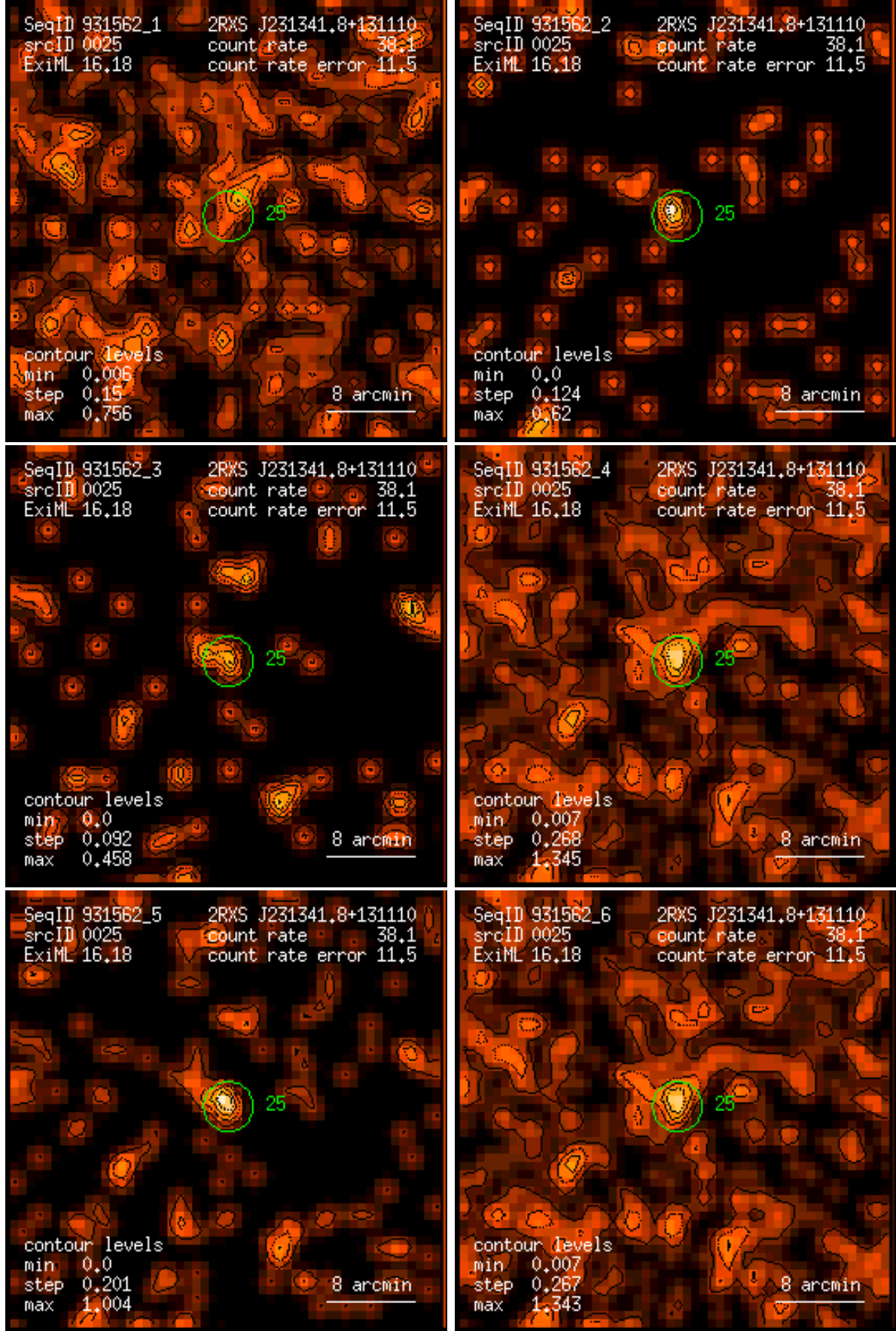
Figure 25: RASS 931562: detection 0025: band rate images, Gaussian filter: (1) PSPC channels 11 – 41, (2) 52 – 90, (3) 91 – 201, (4) 11 – 235, (5) 52 – 201, (6) 11 – 201. Broad band rates in counts/ks. Band rate contour levels in counts/ks/arcmin 2 .
