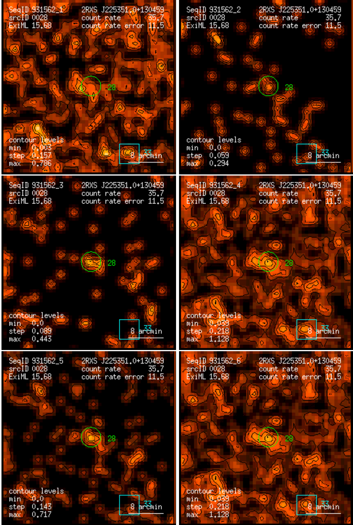
Figure 28: RASS 931562: detection 0028: band rate images, Gaussian filter: (1) PSPC channels 11 – 41, (2) 52 – 90, (3) 91 – 201, (4) 11 – 235, (5) 52 – 201, (6) 11 – 201. Broad band rates in counts/ks. Band rate contour levels in counts/ks/arcmin 2 .
