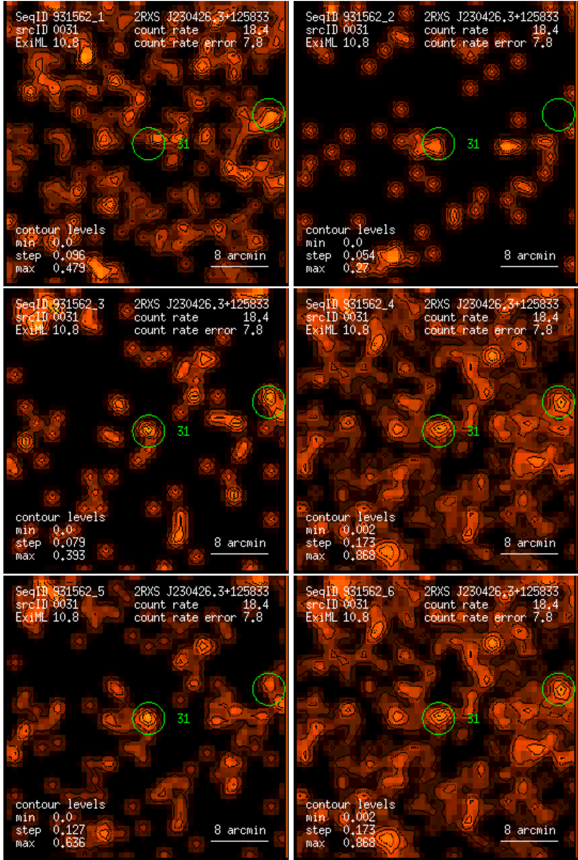
Figure 31: RASS 931562: detection 0031: band rate images, Gaussian filter: (1) PSPC channels 11 – 41, (2) 52 – 90, (3) 91 – 201, (4) 11 – 235, (5) 52 – 201, (6) 11 – 201. Broad band rates in counts/ks. Band rate contour levels in counts/ks/arcmin 2 .
