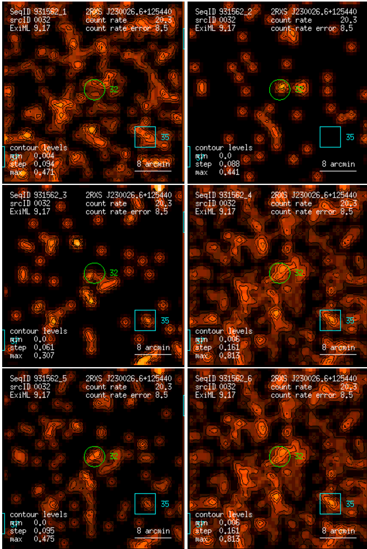
Figure 32: RASS 931562: detection 0032: band rate images, Gaussian filter: (1) PSPC channels 11 – 41, (2) 52 – 90, (3) 91 – 201, (4) 11 – 235, (5) 52 – 201, (6) 11 – 201. Broad band rates in counts/ks. Band rate contour levels in counts/ks/arcmin 2 .
