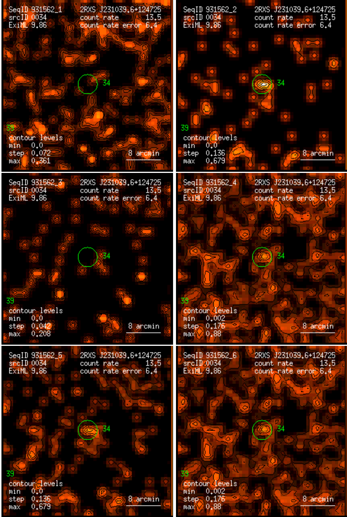
Figure 34: RASS 931562: detection 0034: band rate images, Gaussian filter: (1) PSPC channels 11 – 41, (2) 52 – 90, (3) 91 – 201, (4) 11 – 235, (5) 52 – 201, (6) 11 – 201. Broad band rates in counts/ks. Band rate contour levels in counts/ks/arcmin 2 .
